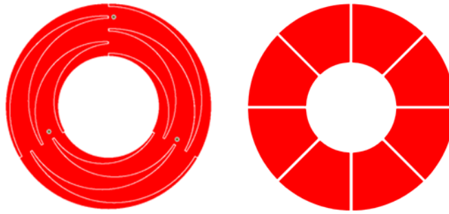
Figure 32. Metal Wheel Sensor Patterns
