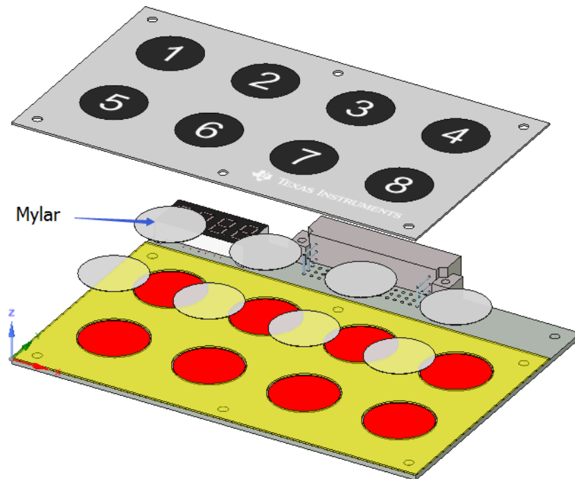
Figure 37. Mylar to Protect Electrodes
