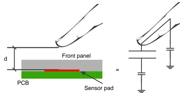
Figure 4. Theory of Capacitive Touch
