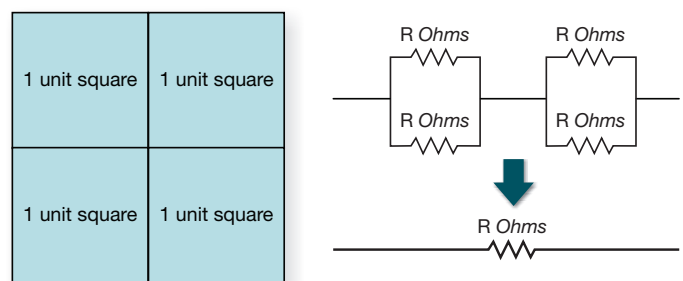
Figure 7. Sheet resistance for four squares.
