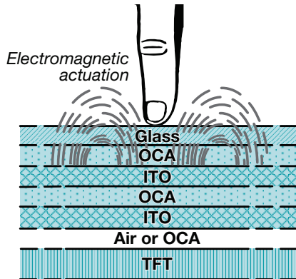
Figure 5. ITO capacitive-touch sensor with TFT LCD.
