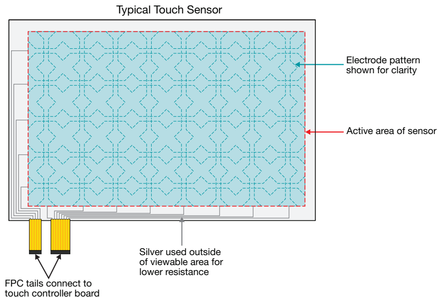
Figure 1. Typical touch sensor structure.
