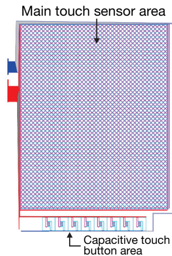
Figure 2. Touch screen with capacitive buttons.
