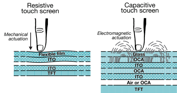
Figure 4. An ITO resistive-touch sensor vs. an ITO capacitive-touch sensor.
