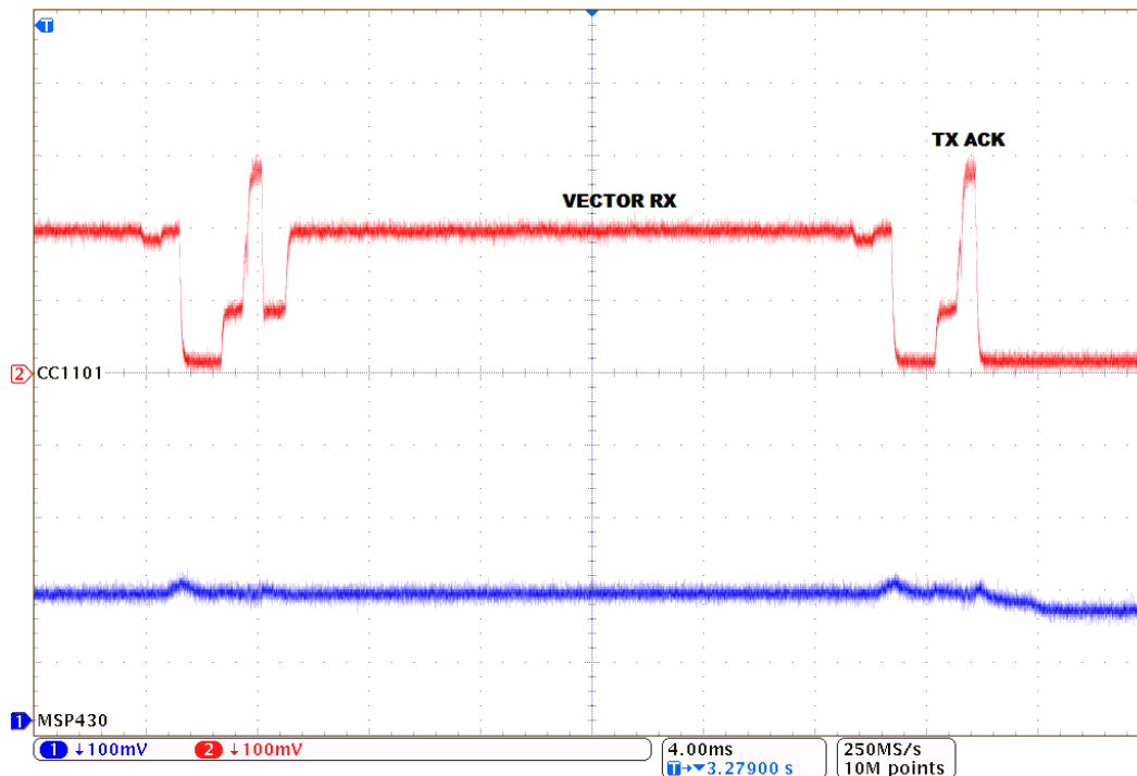
Figure 44. Current Measurement of a Reset Vector Packet
