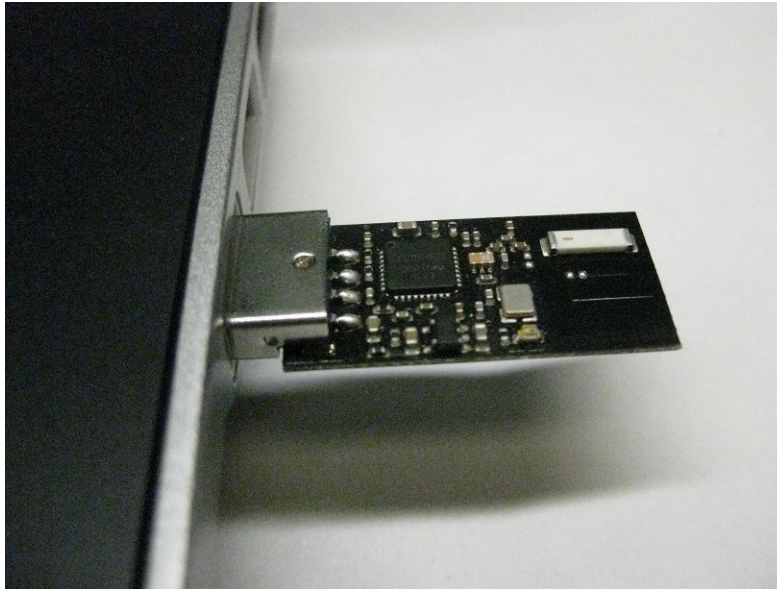
Figure 5. CC1111 USB RF Access Point Connected to USB Port
