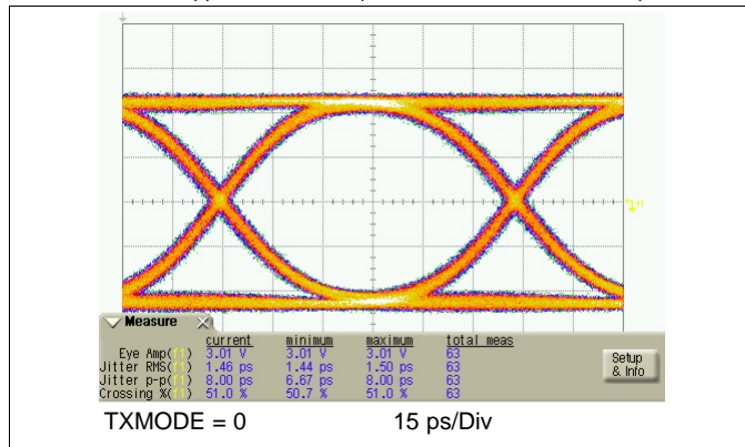
Figure 20. TX Eye-Diagram at 11.3 Gbps
