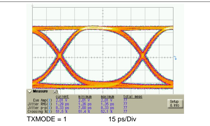
Figure 21. TX Eye-Diagram at 11.3 Gbps
