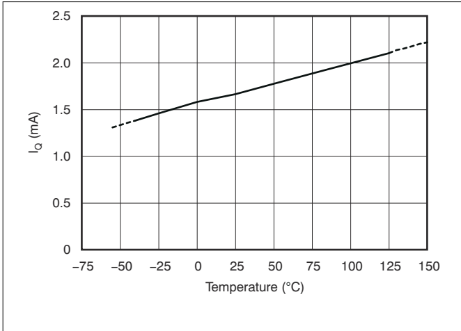
Figure 6-13. Quiescent Current vs Temperature
