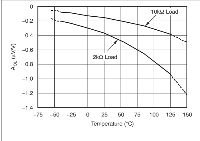
Figure 6-17. Open-Loop Gain vs Temperature
