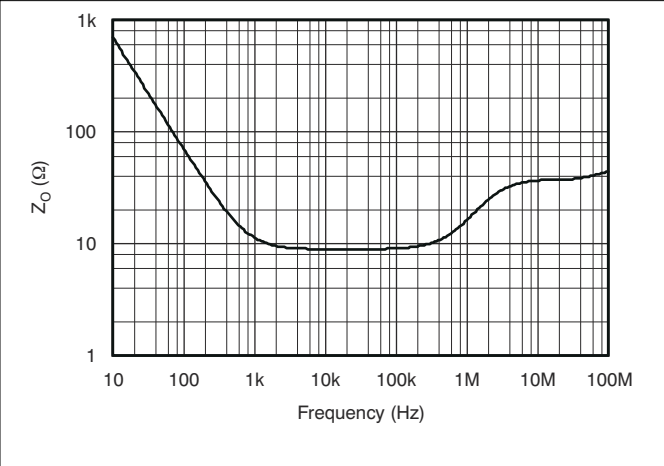
Figure 6-18. Open-Loop Output Impedance vs Frequency
