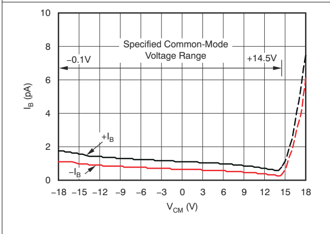
Figure 6-5. I_B vs Common-Mode Voltage
