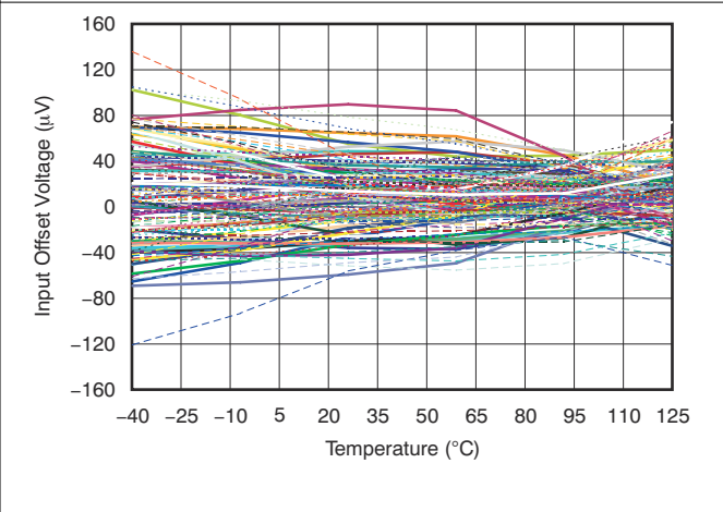
Figure 6-4. Input Offset Voltage vs Temperature (144 Amplifiers)
