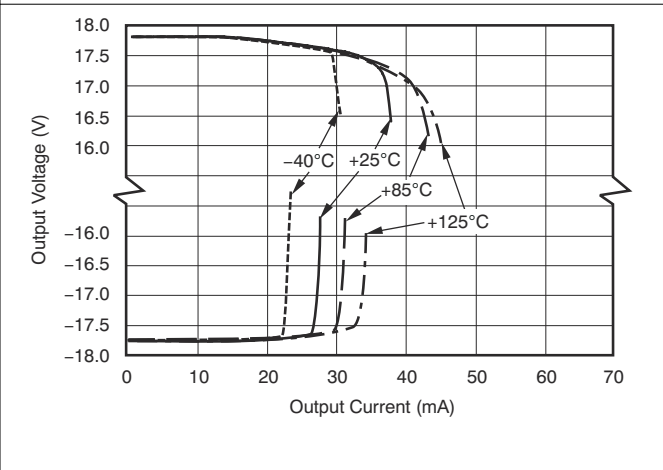
Figure 6-6. Output Voltage Swing vs Output Current (Maximum Supply)
