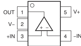
Figure 5-2. OPA140: DBV (5-Pin SOT-23) Package, Top View
