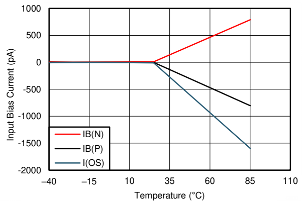
Figure 6-18. I_B and I_{OS} vs Temperature
