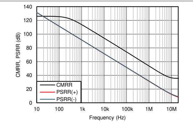
Figure 6-12. CMRR and PSRR vs Frequency (Referred to Input)
