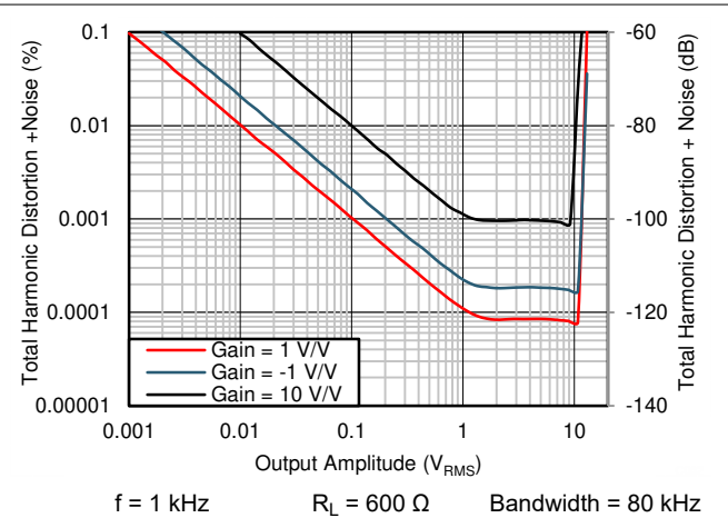
Figure 6-10. THD+N Ratio vs Output Amplitude
