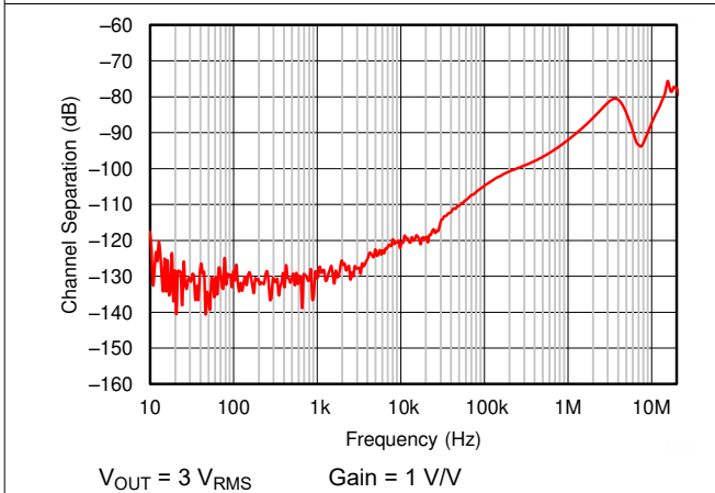
Figure 6-11. Channel Separation vs Frequency
