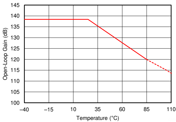
Figure 6-17. Open-Loop Gain vs Temperature
