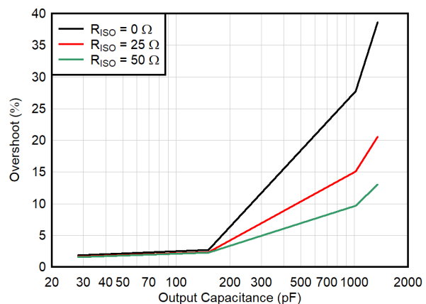
Figure 7-30. Small-Signal Overshoot vs Capacitive Load (10-mV Step)
