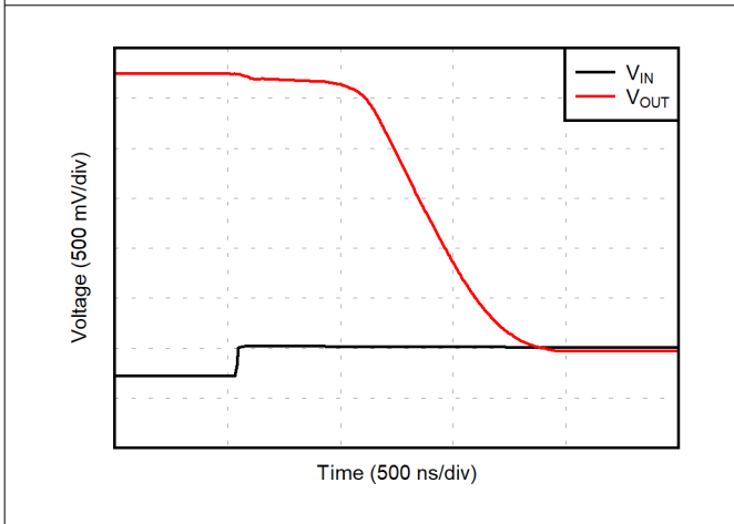
Figure 7-33. Positive Overload Recovery
