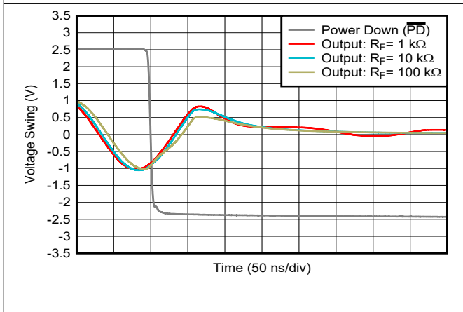
Figure 6-15. Turn-Off Transient Response
