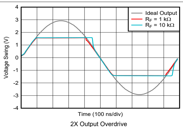
Figure 6-12. Output Overload Response – Low Gain Settings
