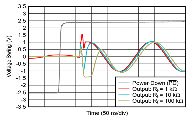
Figure 6-14. Turn-On Transient Response
