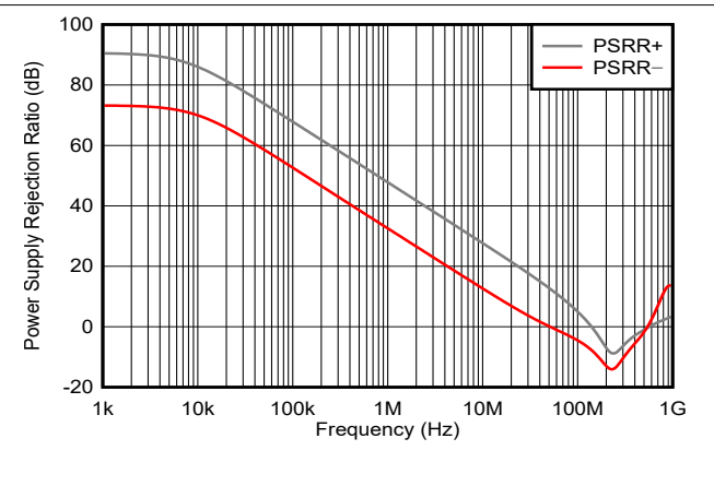
Figure 6-16. Power Supply Rejection Ratio vs Frequency
