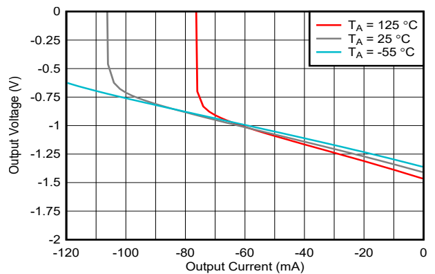
Figure 6-28. Output Swing vs Sinking Current
