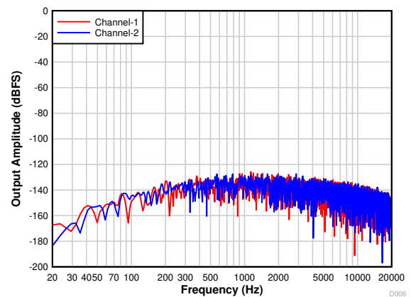
Figure 7-18. PCM1821-Q1: FFT With Idle Input and DRE Disabled
