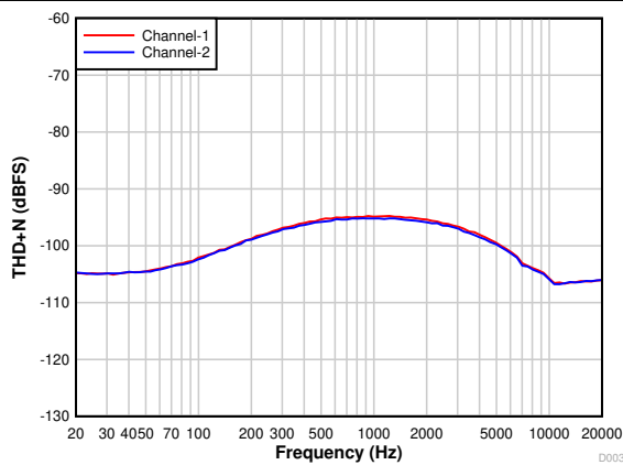
Figure 7-15. PCM1821-Q1: THD+N vs Input Frequency With a -1-dBr Input
