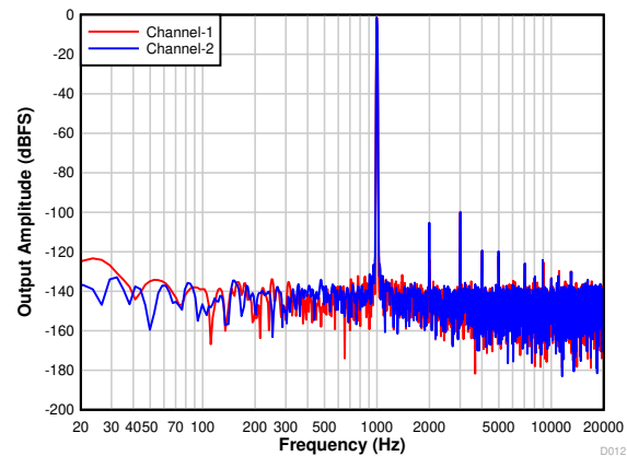
Figure 7-12. PCM1820-Q1: FFT With a -1-dBr Input
