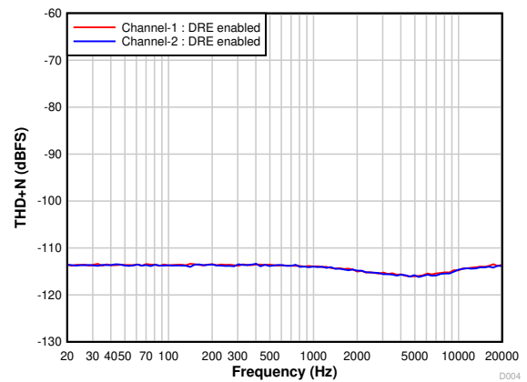
Figure 7-4. PCM1820-Q1: THD+N vs Input Frequency With a -60-dBr Input
