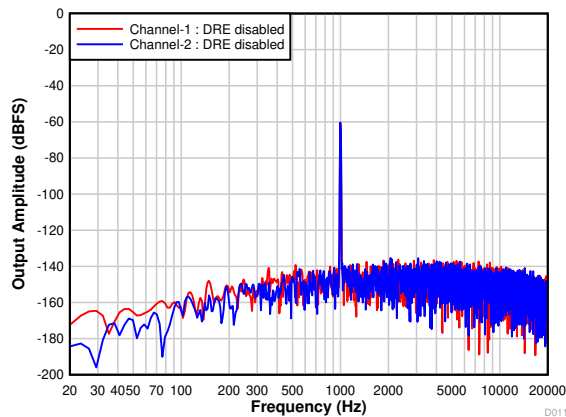
Figure 7-11. PCM1820-Q1: FFT With a -60-dBr Input and DRE Disabled
