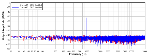
Figure 9-4. PCM1820-Q1: FFT With a -60-dBr Input With DRE Disabled
