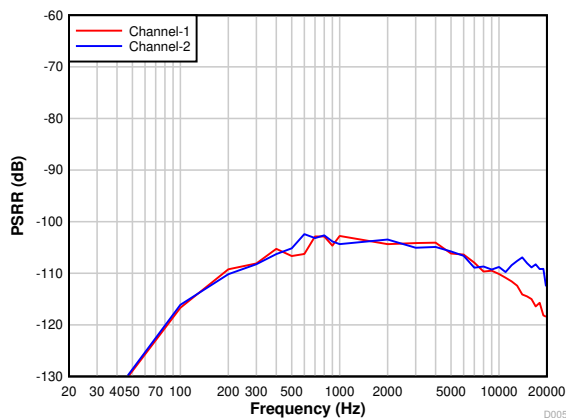
Figure 7-17. PCM1821-Q1: Power-Supply Rejection Ratio vs Ripple Frequency With a 100-mV PP Amplitude
