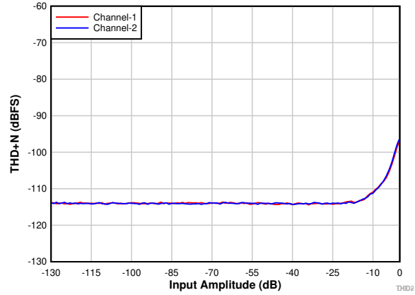
Figure 7-2. PCM1820-Q1: THD+N vs Input Amplitude With DRE Disabled
