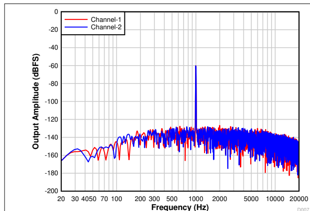
Figure 7-19. PCM1821-Q1: FFT With a -60\text{-dBr} Input and DRE Enabled
