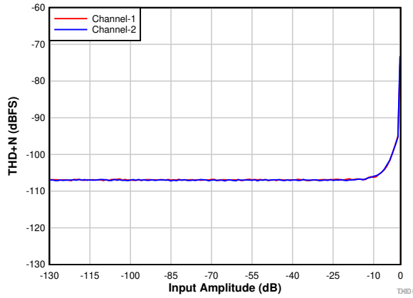
Figure 7-13. PCM1821-Q1: THD+N vs Input Amplitude
