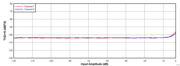
Figure 9-7. PCM1821-Q1: THD+N vs Input Amplitude
