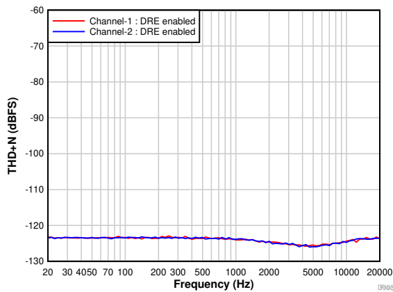
Figure 7-3. PCM1820-Q1: THD+N vs Input Frequency With a -60-dBr Input
