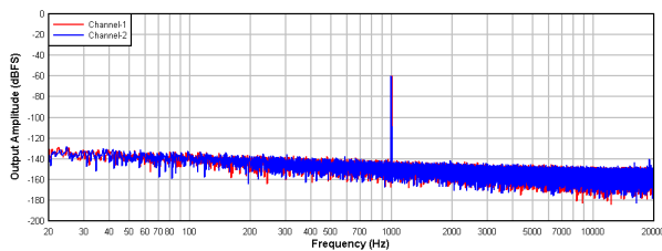
Figure 9-6. PCM1821-Q1: FFT With a -60-dBr Input
