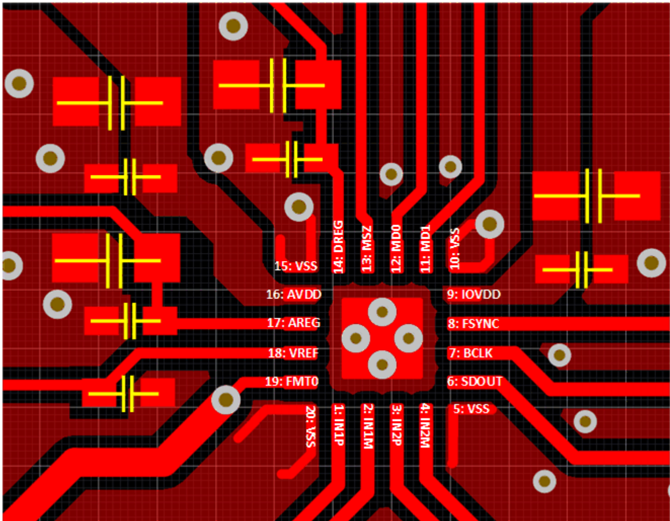
Figure 11-1. Example Layout
