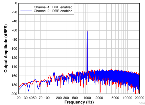
Figure 7-10. PCM1820-Q1: FFT With a -60-dBr Input and DRE Enabled
