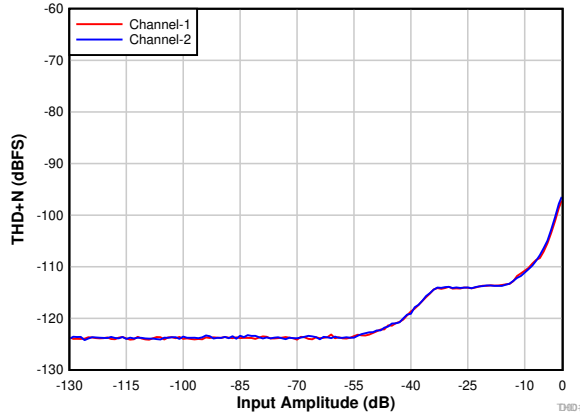
Figure 7-1. PCM1820-Q1: THD+N vs Input Amplitude With DRE Enabled
