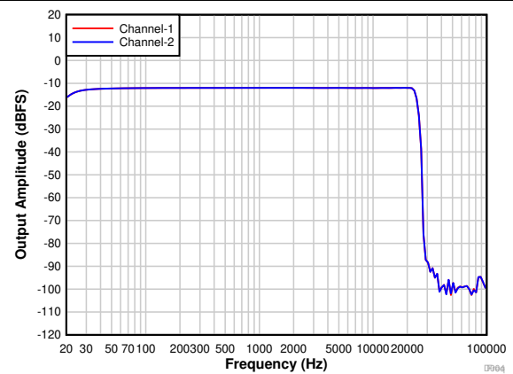
Figure 7-16. PCM1821-Q1: Frequency Response With a -12-dBr Input
