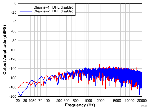
Figure 7-9. PCM1820-Q1: FFT With Idle Input and DRE Disabled
