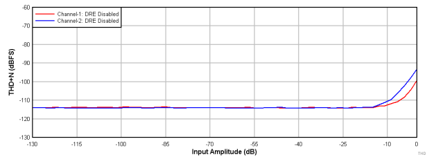
Figure 9-5. PCM1820-Q1: THD+N vs Input Amplitude With DRE Disabled
