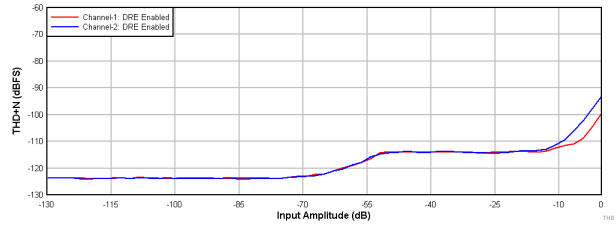
Figure 9-3. PCM1820-Q1: THD+N vs Input Amplitude With DRE Enabled
