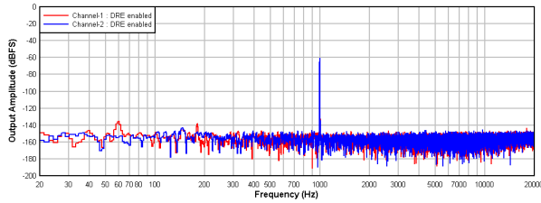
Figure 9-2. PCM1820-Q1: FFT With a -60-dBr Input With DRE Enabled
