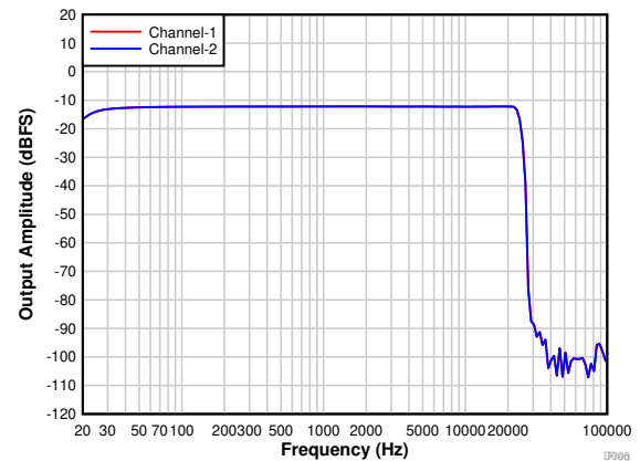
Figure 7-6. PCM1820-Q1: Frequency Response With a -12-dBr Input
