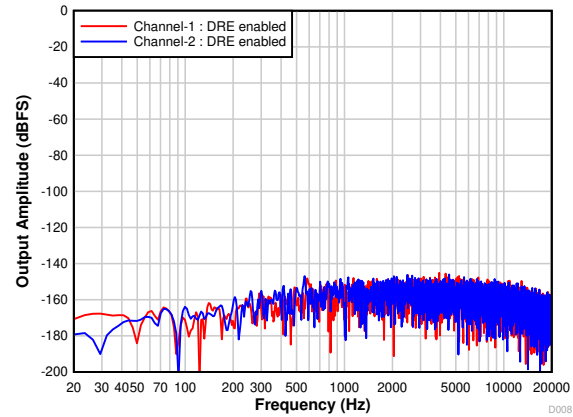
Figure 7-8. PCM1820-Q1: FFT With Idle Input and DRE Enabled
