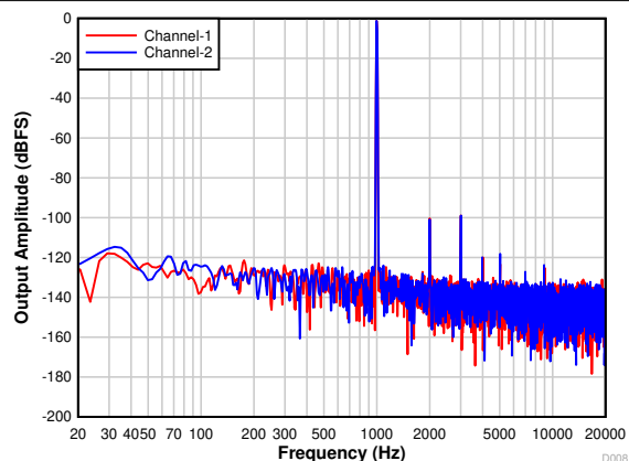
Figure 7-20. PCM1821-Q1: FFT With a -1\text{-dBr} Input
