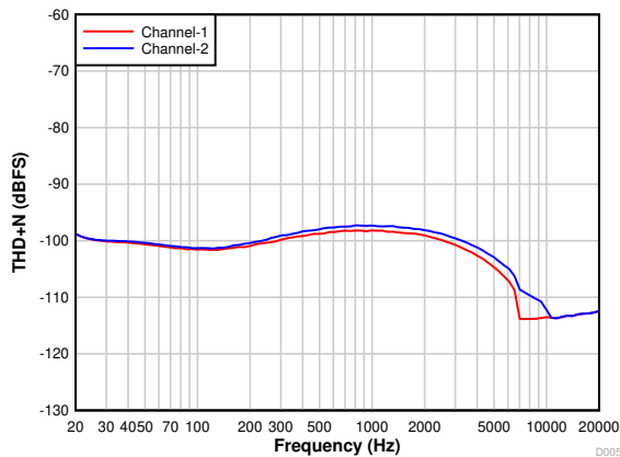
Figure 7-5. PCM1820-Q1: THD+N vs Input Frequency With a -1-dBr Input
