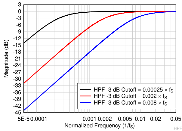
Figure 8-17. HPF Filter Frequency Response Plot
