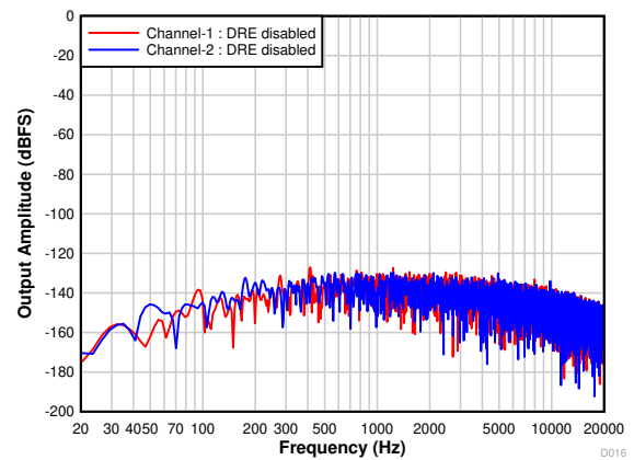
Figure 7-19. FFT With Idle Input With DRE Disabled
