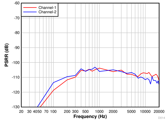
Figure 7-17. Power-Supply Rejection Ratio vs Ripple Frequency With 100-mV pp Amplitude
