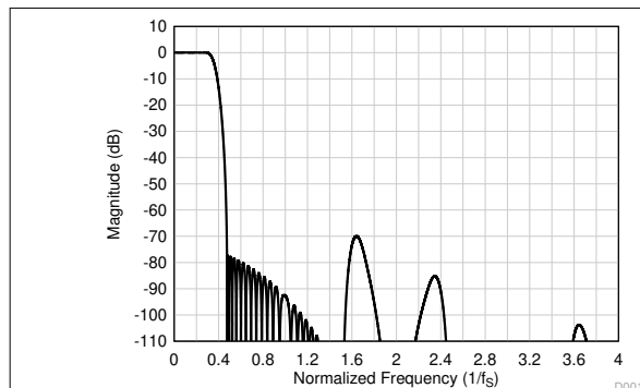
Figure 8-31. Linear Phase Decimation Filter Magnitude Response
