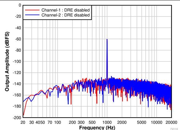
Figure 7-21. FFT With a -60-dBr Input With DRE Disabled
