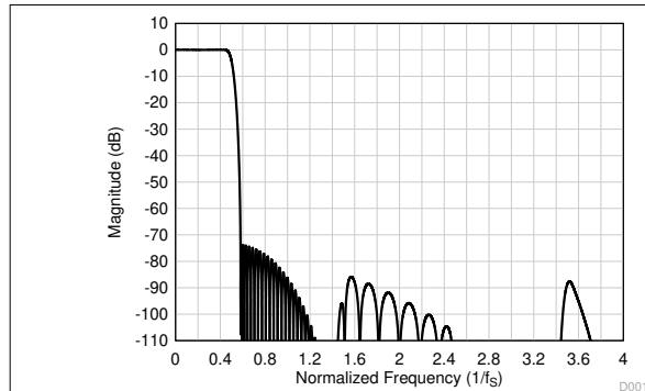
Figure 8-29. Linear Phase Decimation Filter Magnitude Response
