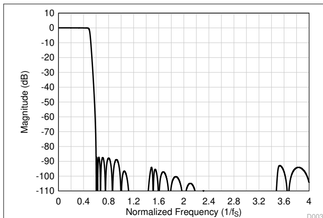
Figure 7-49. Ultra-Low-Latency Decimation Filter Magnitude Response
