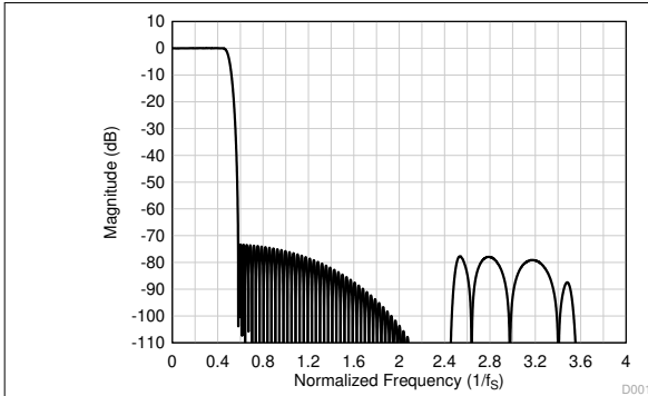
Figure 7-21. Linear Phase Decimation Filter Magnitude Response
