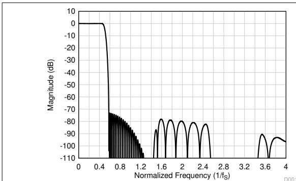
Figure 7-23. Linear Phase Decimation Filter Magnitude Response
