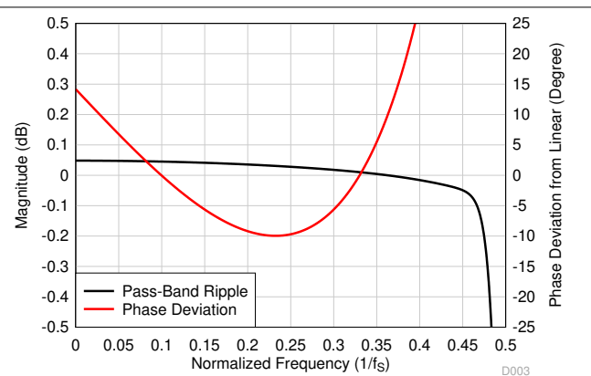
Figure 7-50. Ultra-Low-Latency Decimation Filter Pass-Band Ripple and Phase Deviation
