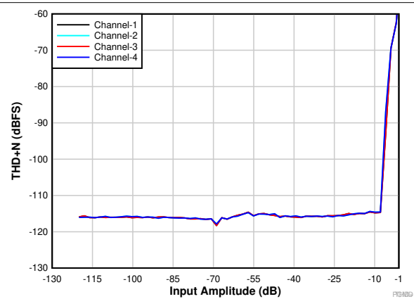
4th-order PDM modulator with PDMCLKx = 2.8224 MHz
