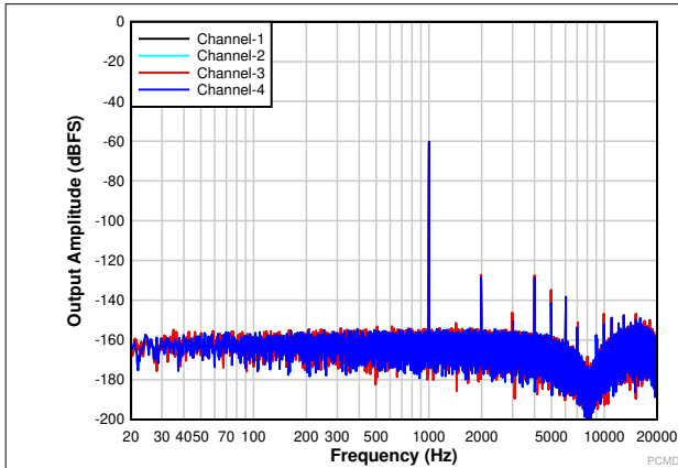
4th-order PDM modulator with PDMCLKx = 2.8224 MHz
