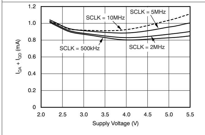
Figure 29. Total Quiescent Current vs Supply Voltage
