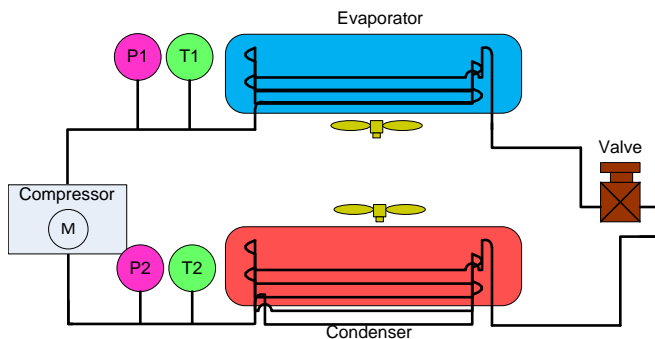
Figure 1. HVAC System
