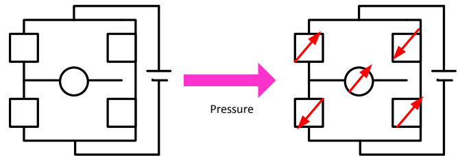
Figure 2. Resistive Bridge
