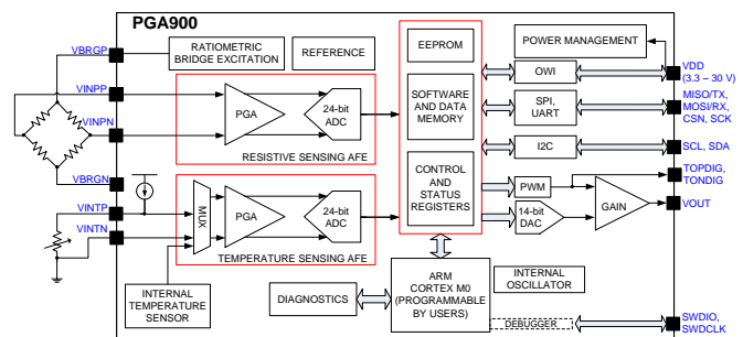
Figure 3. PGA900 Block Diagram
