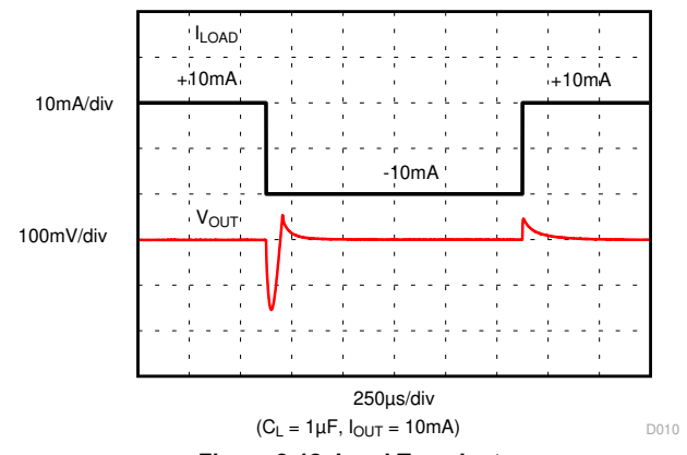
Figure 8-12. Load Transient
