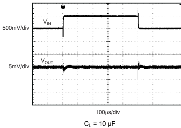
Figure 7-21. Line Transient
