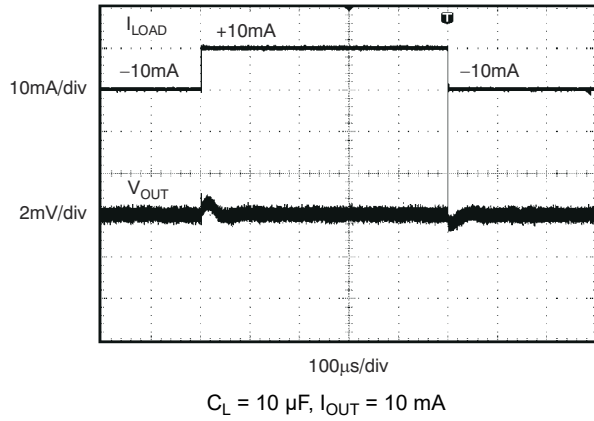
Figure 7-19. Load Transient
