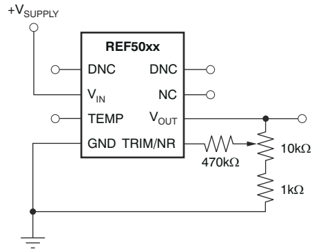
Figure 9-3. V OUT Adjustment Using the TRIM/NR Pin
