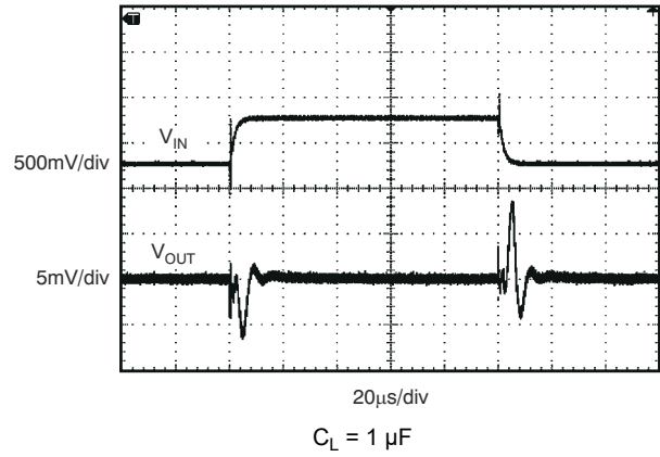
Figure 7-20. Line Transient
