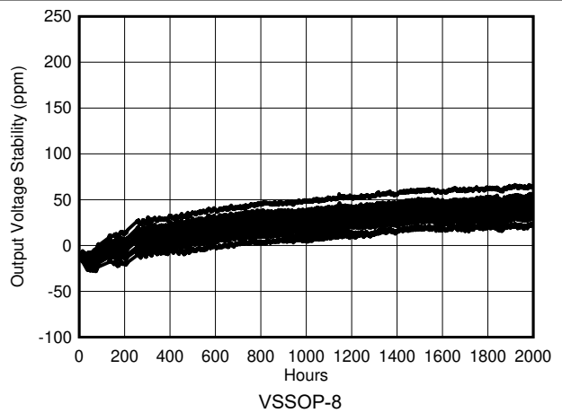
Figure 7-24. REF50xx Long-Term Stability (First 2000 Hours)
