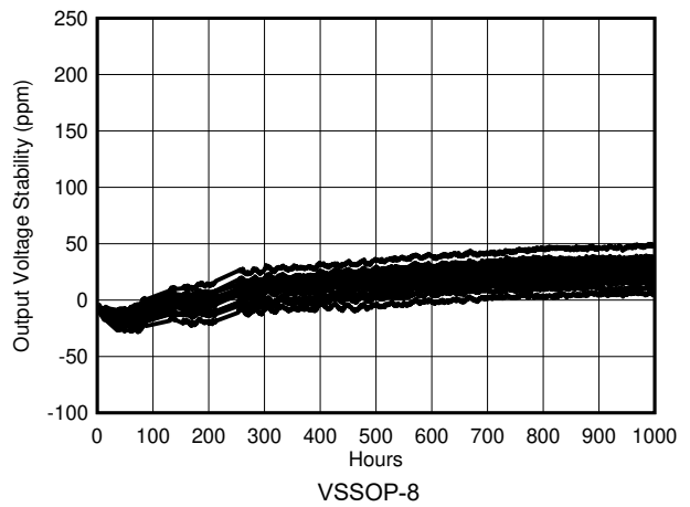
Figure 7-22. REF50xx Long-Term Stability (First 1000 Hours)
