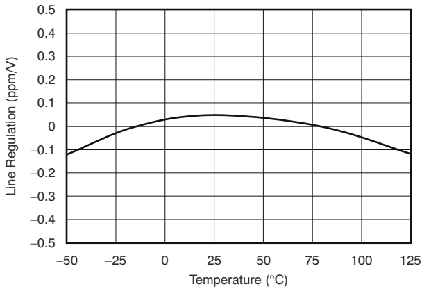
Figure 7-11. Line Regulation vs Temperature
