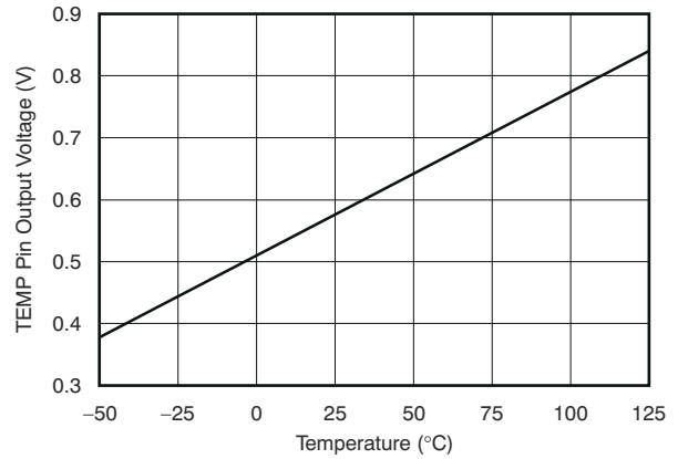
Figure 7-8. Temp Pin Output Voltage vs Temperature
