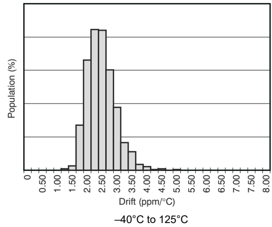
Figure 7-2. Temperature Drift
