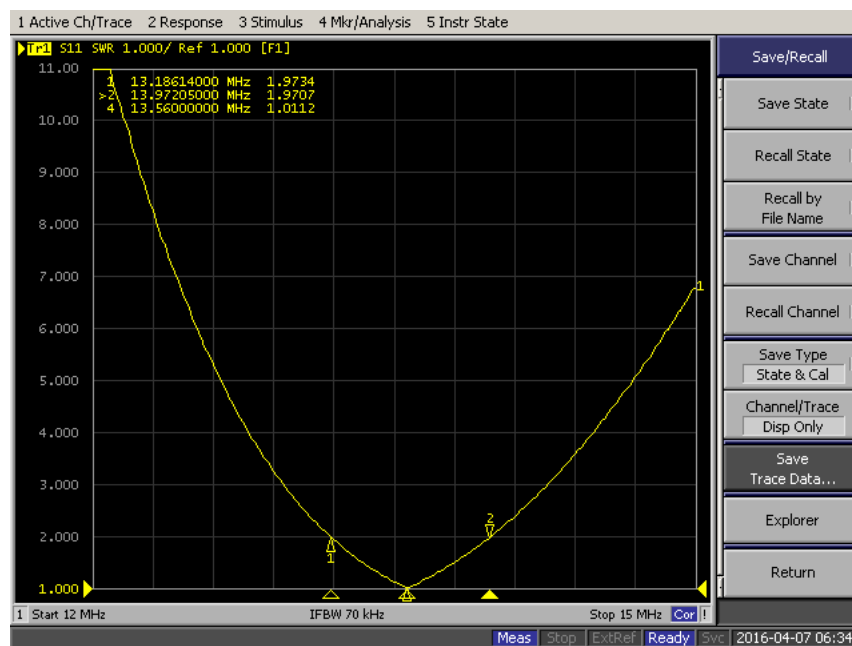
Figure 6. Tuned 5-mm x 5-mm Antenna Standing Wave Ratio
