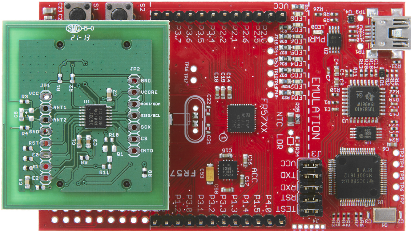
Figure 1. RF430CL330HTB + MSP-EXP430FR5739
