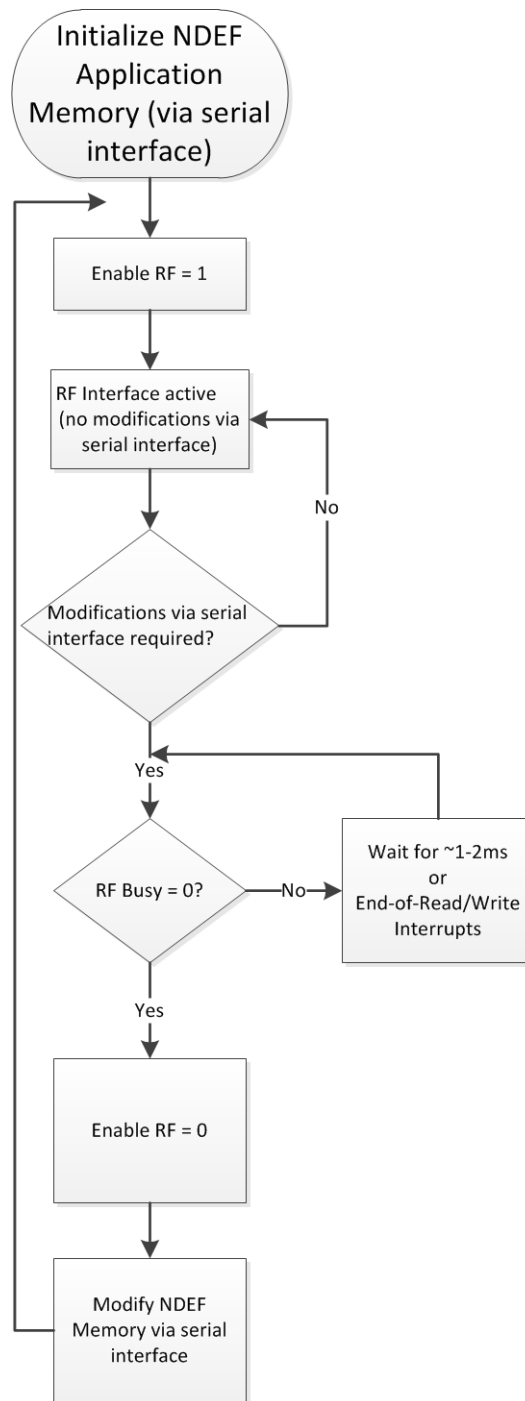
Figure 7. Recommended Firmware Flow
