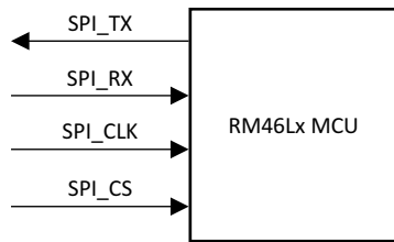
Figure 1. SPI Connections for RM46 Bootloader
