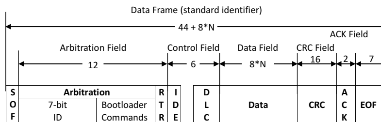
Figure 3. Standard CAN Frame Format
