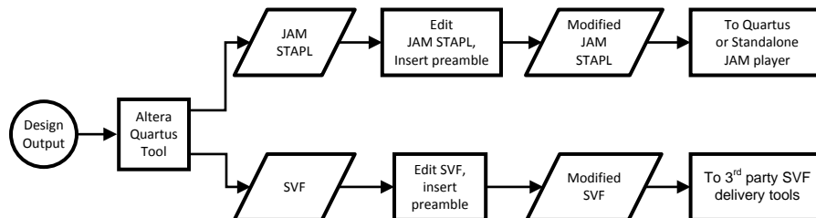
Figure 2. Tool Chain and Process for Modifying JAM STAPL or SVF
