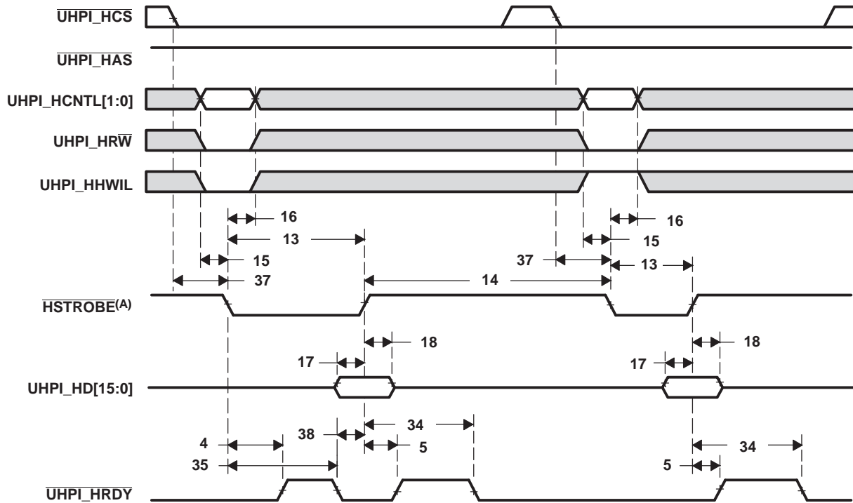
Figure 4-23. Multiplexed Read Timings With \overline{\text{UHPI\_HAS}} Held High
