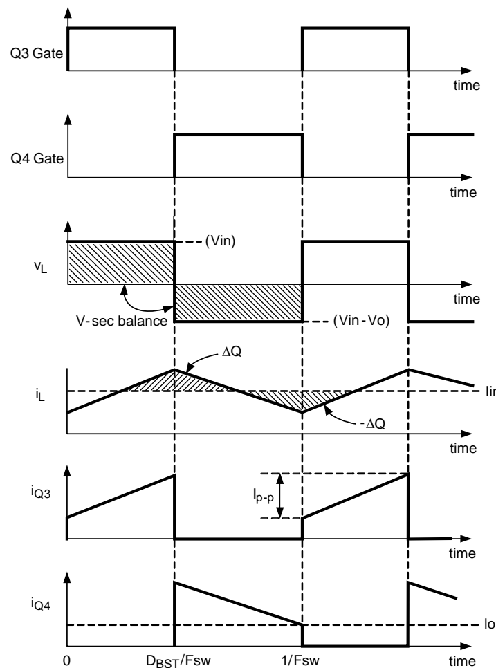
Figure 9. Boost-Only Key Waveforms
