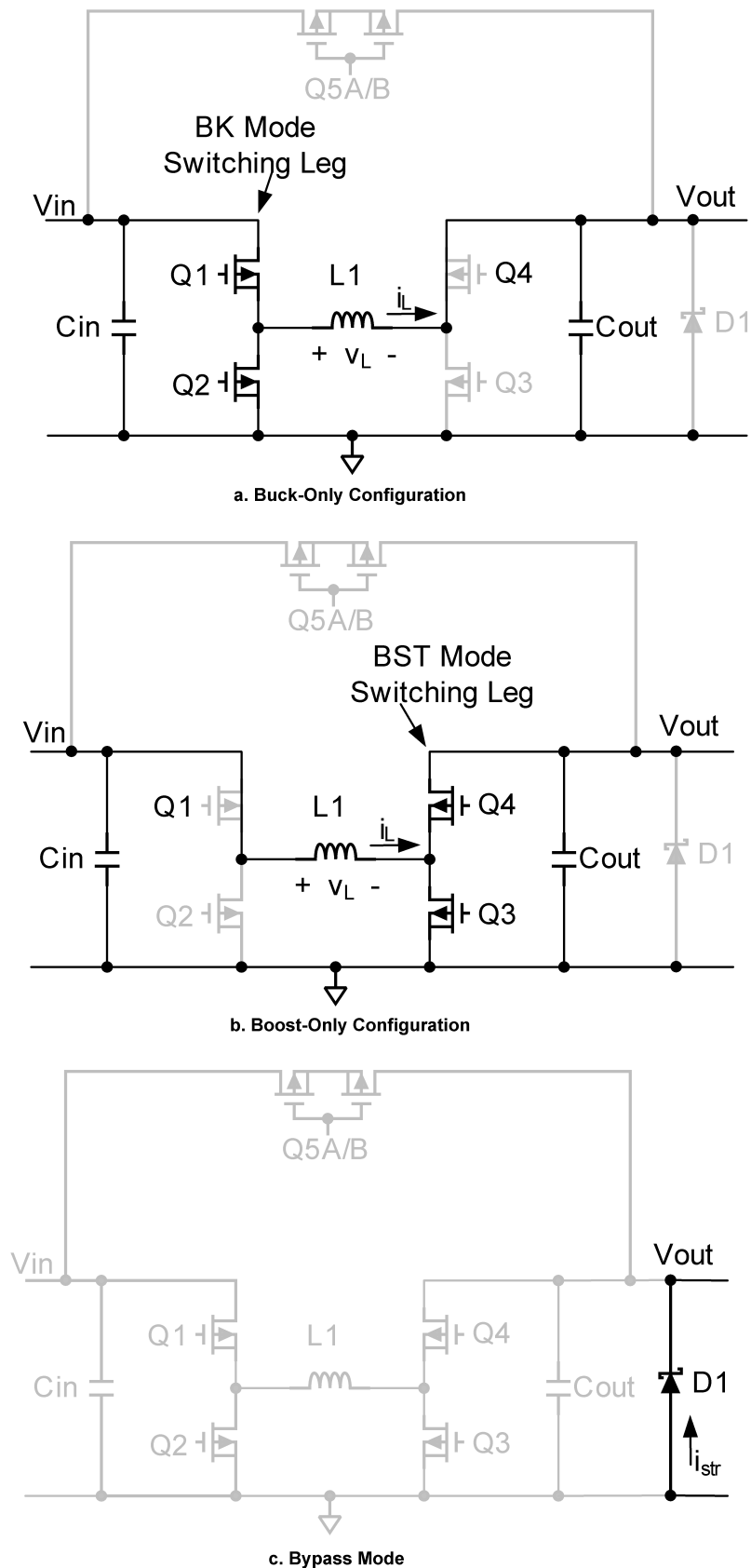
Figure 7. Buck-Only, Boost-Only and Output Bypass Configurations
