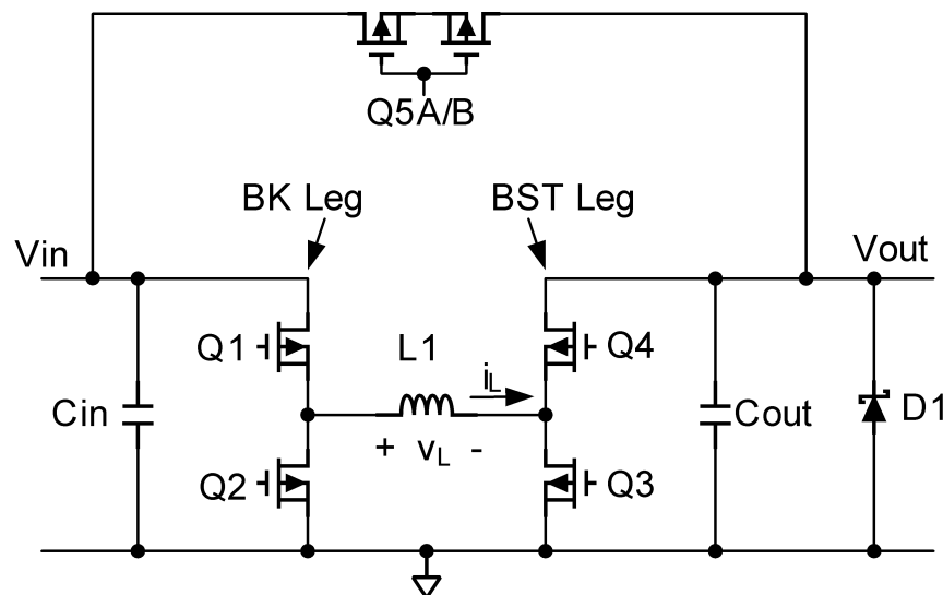
Figure 5. Buck-and-Boost Converter Topology With Panel Mode Switch
