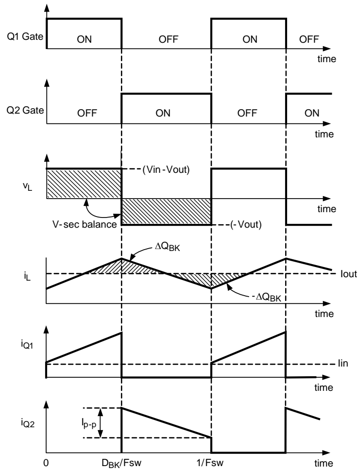
Figure 8. Buck-Only Key Waveforms
