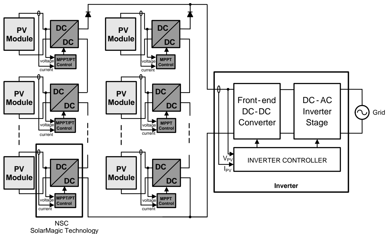
Figure 1. SolarMagic MPPT/PM Enhanced PV System Architecture
