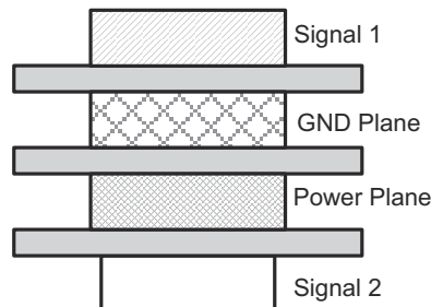
Figure 11-2. Example Layout
