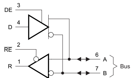
Figure 13. Half-Duplex Transceiver
