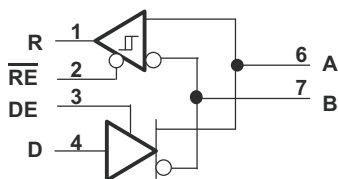
Figure 27. Logic Diagram
