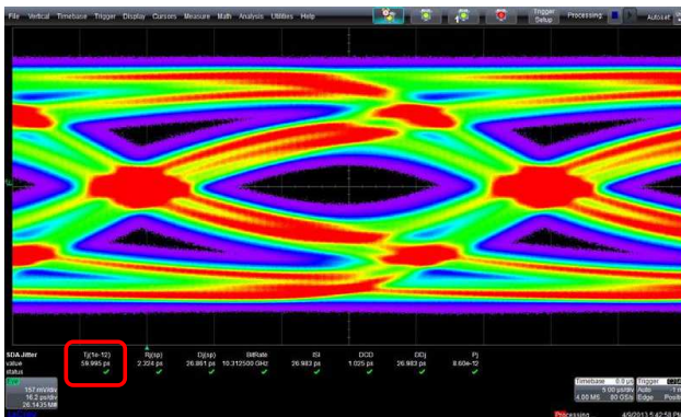
Figure 17. 4" x 4mil Channel No Equalizer Present (~3.5dB Loss)
