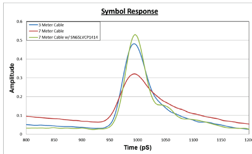
Figure 6. Symbol Response
