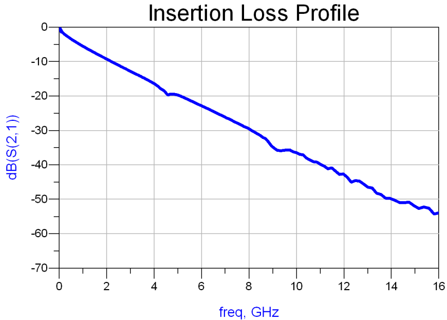
Figure 1. Insertion Loss (SDD21) – 24in x 4mil Trace
