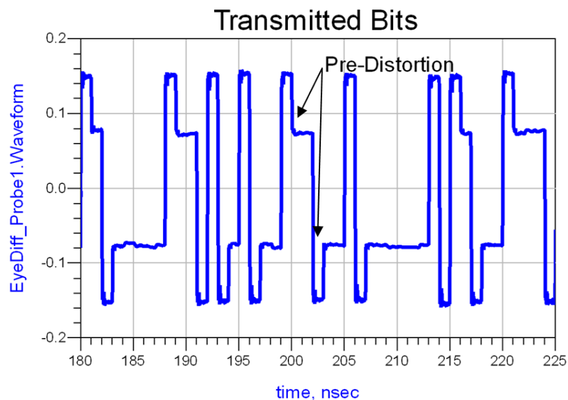
Figure 3. Transmit Equalization
