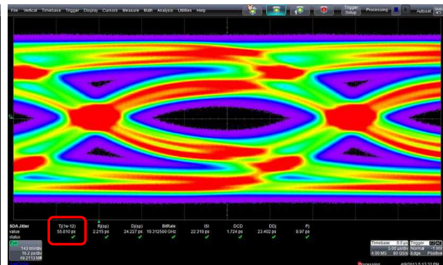
Figure 18. 4" x 4mil Channel – Equalizer Present (Eq=0/-3.5dB Loss)
