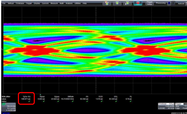
Figure 19. 8" x 4mil Channel – No Equalizer Present (>1UI of Total Jitter/~6dB of Loss)
