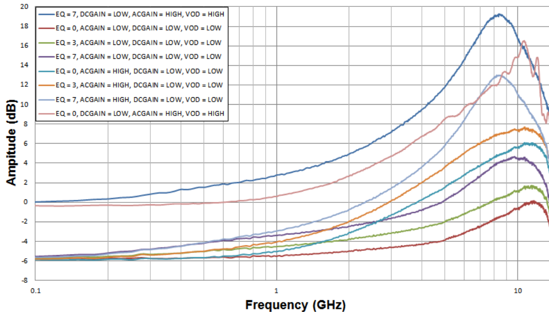
Figure 5. SN65LVCP141x Gain Profile Curves
