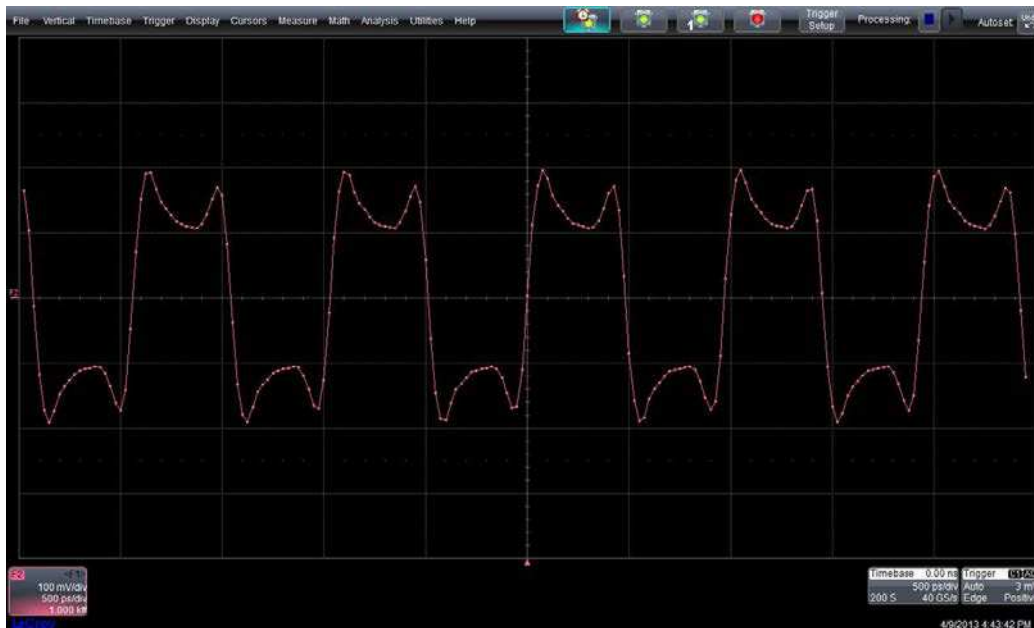
Figure 16. Pre Cursor & Post Cursor Taps Applied to Channel & Linear Equalizer with 6.6dB of Loss
