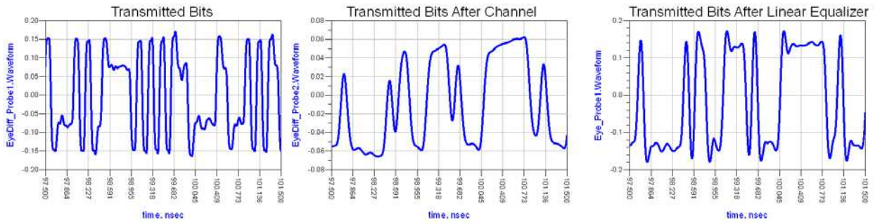
Figure 9. Pre Cursor and Post Cursor Taps Applied to Channel with Linear Equalizer Present
