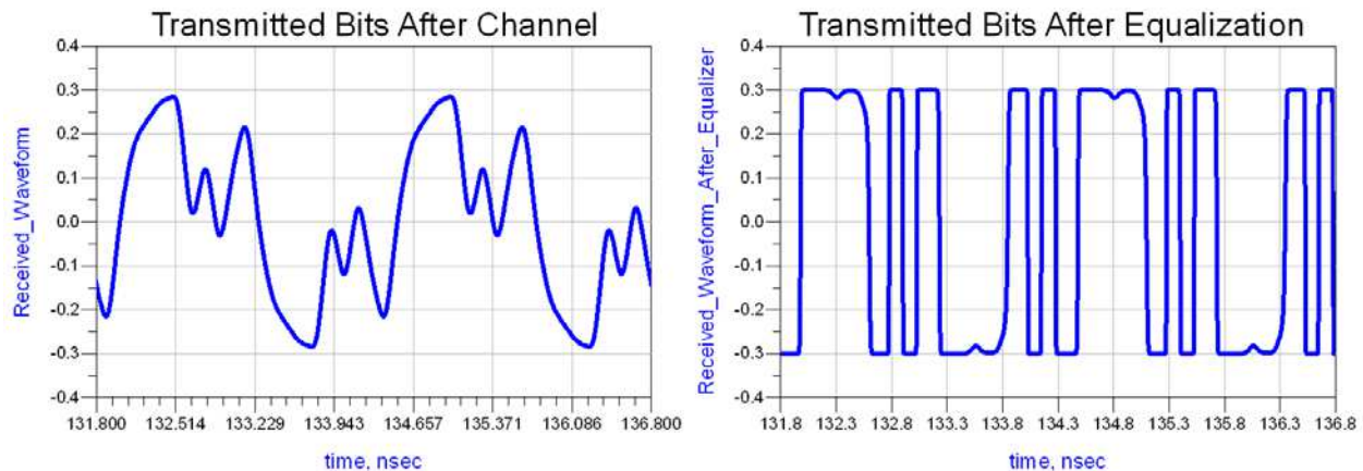
Figure 4. Receive Equalization
