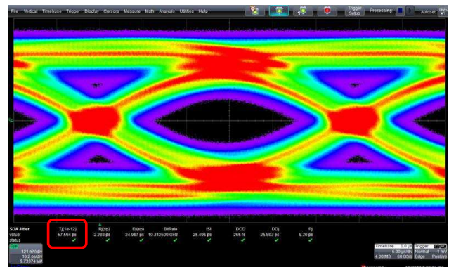
Figure 22. 16" x 4mil Channel – Equalizer Present (AC Gain Medium/Eq=2/Driver Peaking Enabled/~13dB of Loss)
