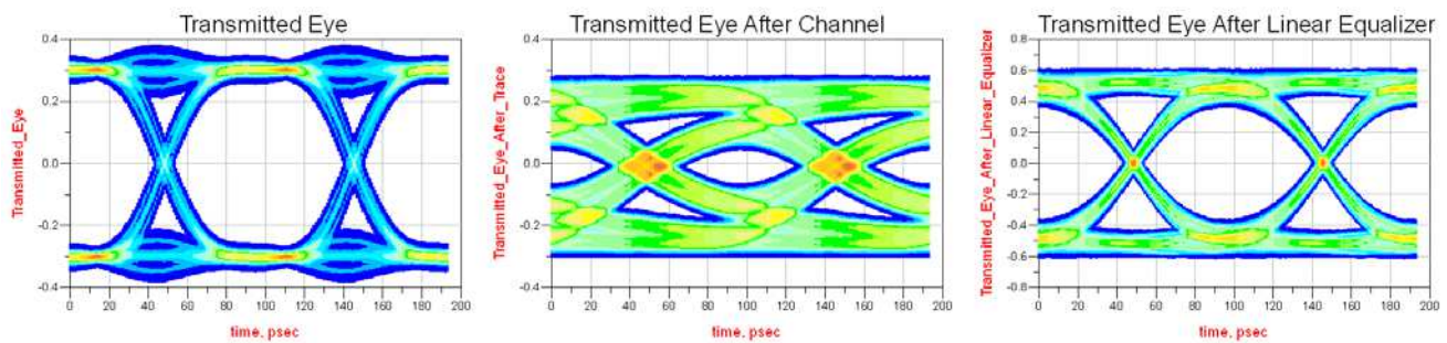
Figure 11. Eye Diagram - 8in x 4mil Trace
