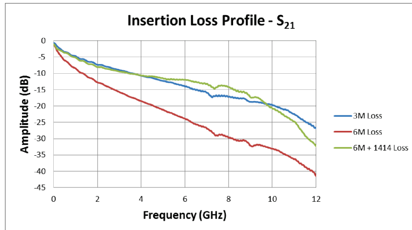
Figure 7. Insertion Loss Profile - S21
