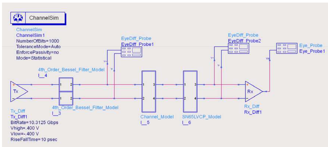
Figure 8. ADS Test Bench
