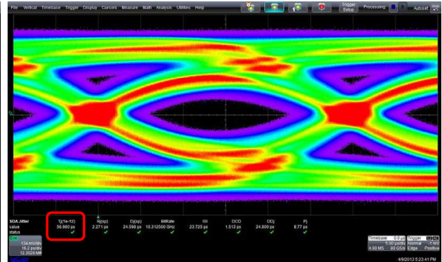
Figure 20. 8" x 4mil Channel – Equalizer Present (0 EQ Implemented/AC Gain Set to Medium/~6dB of Loss)
