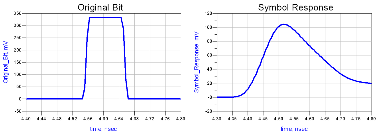
Figure 2. Symbol Response – 24in x 4mil Trace
