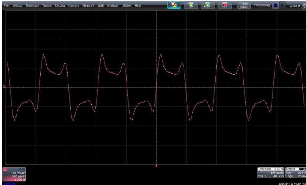
Figure 14. Pre Cursor and Post Cursor Taps Applied to Channel with 3.5dB of Loss
