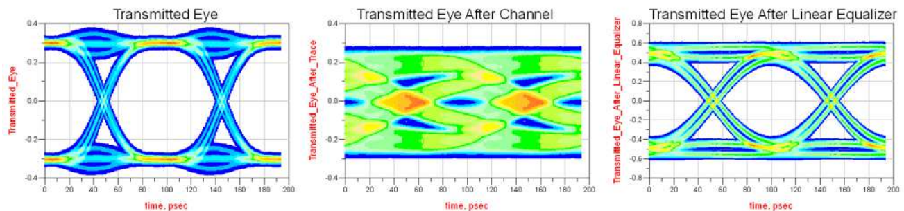
Figure 12. Eye Diagram - 16in x 4mil Trace
