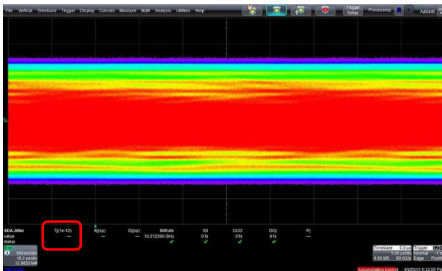
Figure 21. 16" x 4mil Channel – No Equalizer Present (>2UI of Total Jitter/~13dB of Loss)
