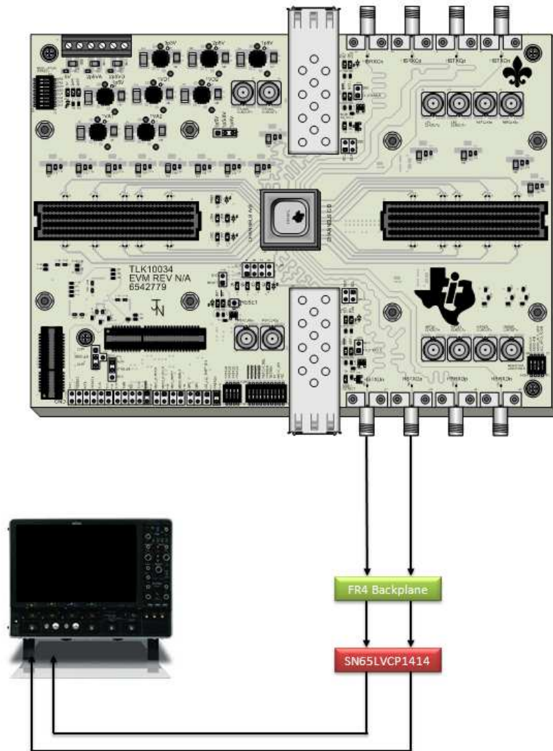
Figure 13. Linear Equalization Test Setup
