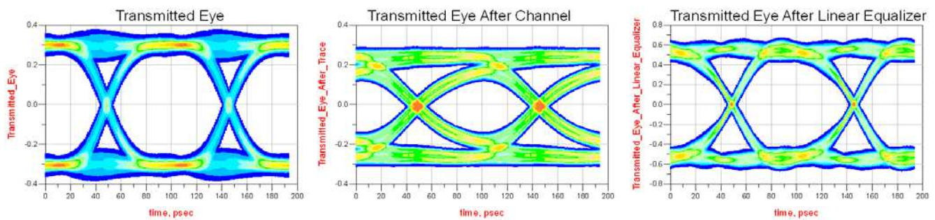
Figure 10. Eye Diagram - 4in x 4mil Trace
