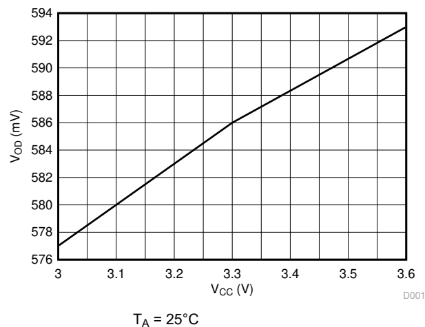
Figure 5-1. Differential Output Voltage vs Supply Voltage
