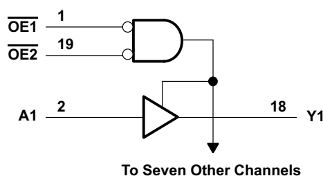
Simplified Block Diagram
