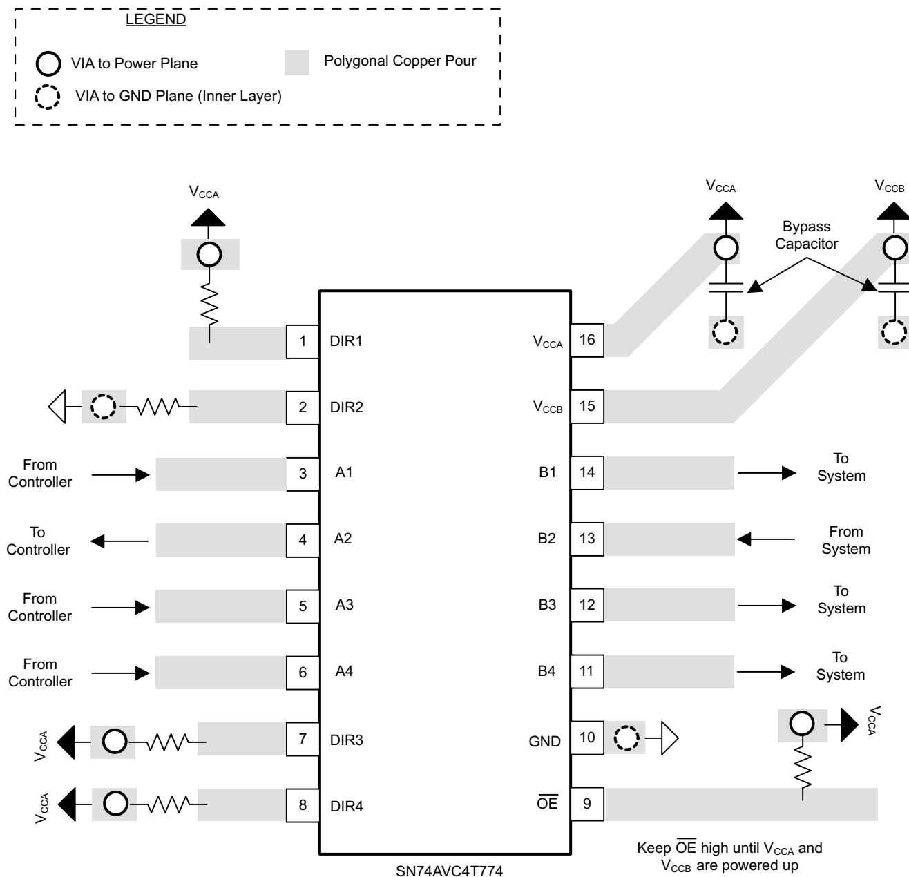
Figure 12-1. PCB Layout Example
