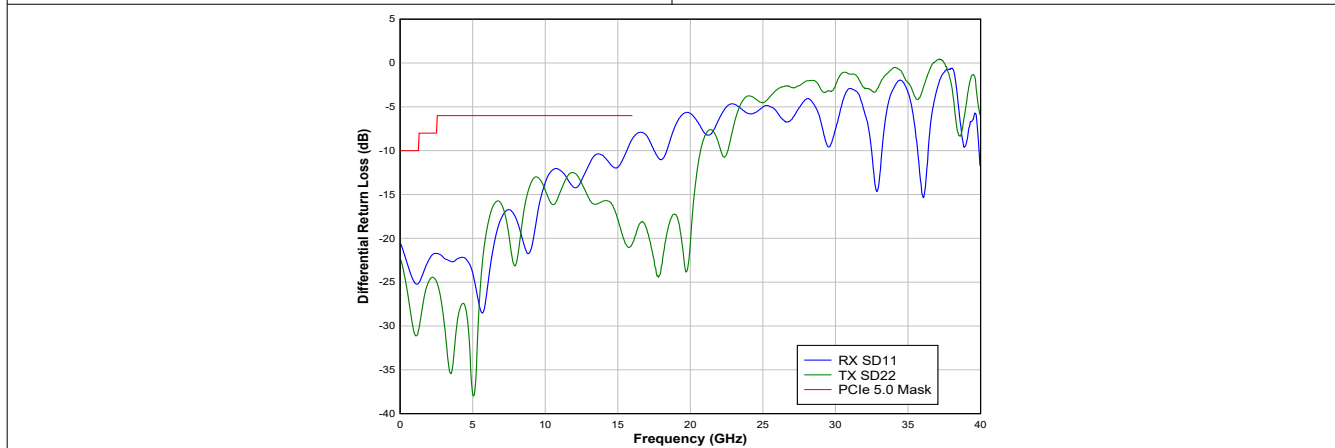
Figure 6-3. Typical Differential Return Loss
