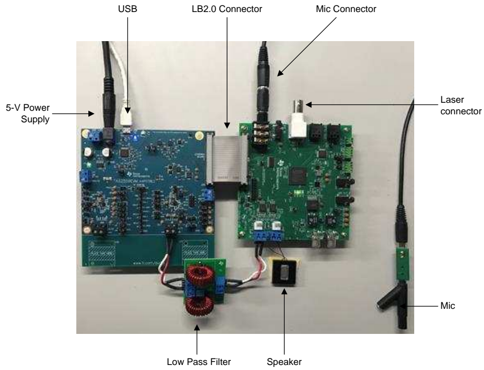
Figure 4. Hardware Setup
