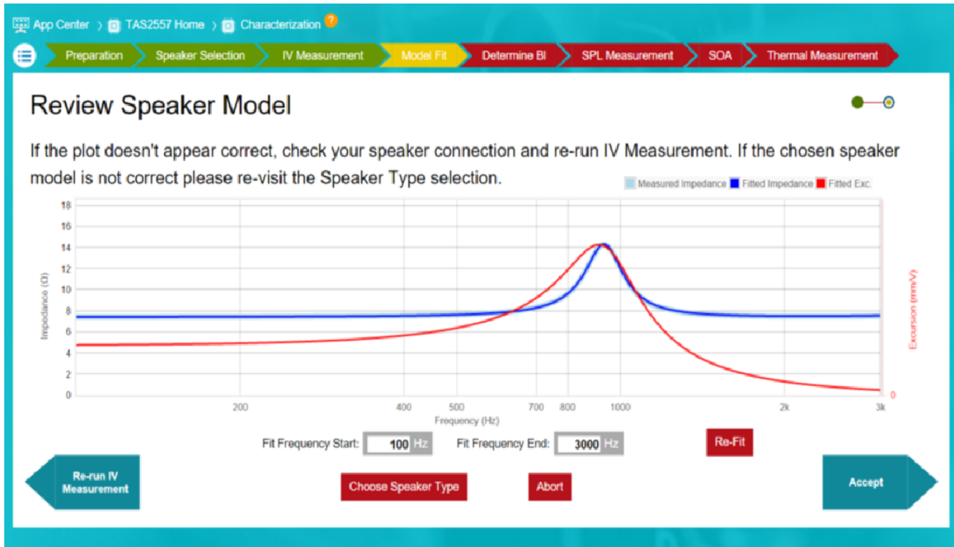
Figure 7. Model Fit
