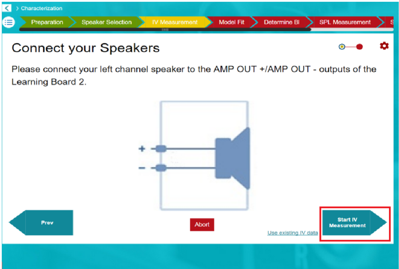
Figure 6. IV Measurement
