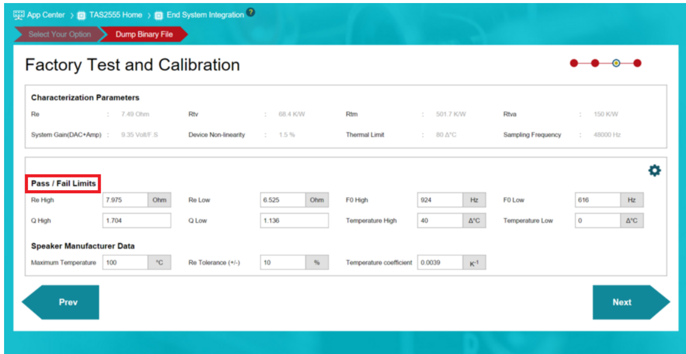
Figure 23. Factory Test and Calibration Step
