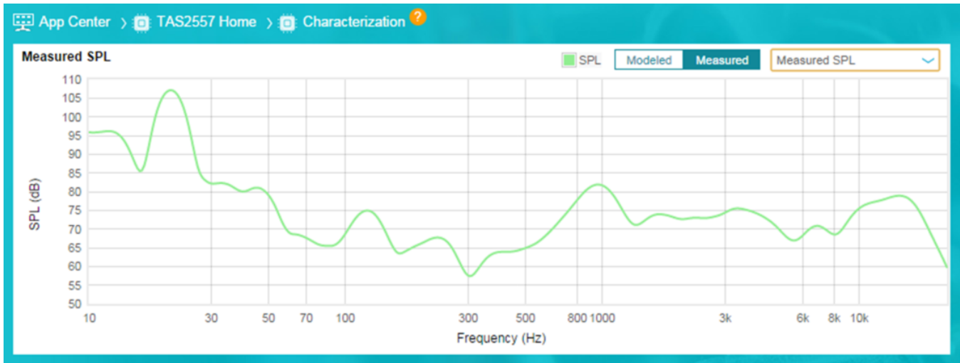
Figure 19. SPL Plot
