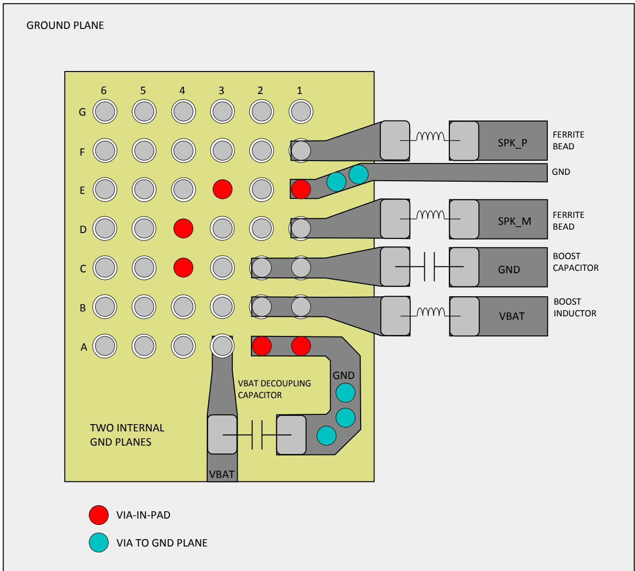
Figure 21. TAS2557 Layout Example
