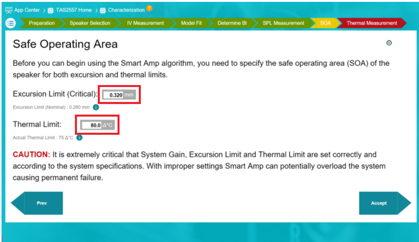
Figure 11. Safe Operating Area
