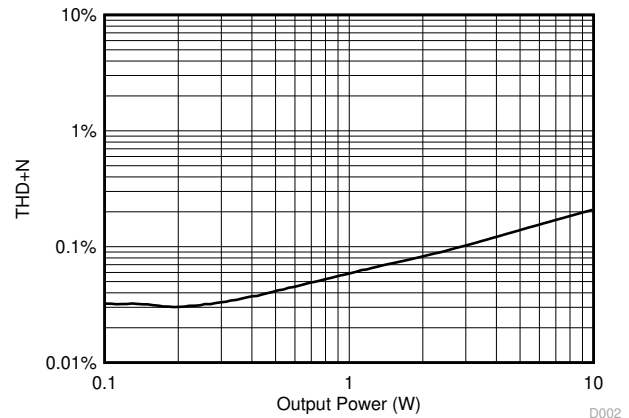
Figure 6-2. THD+N vs Output Power
