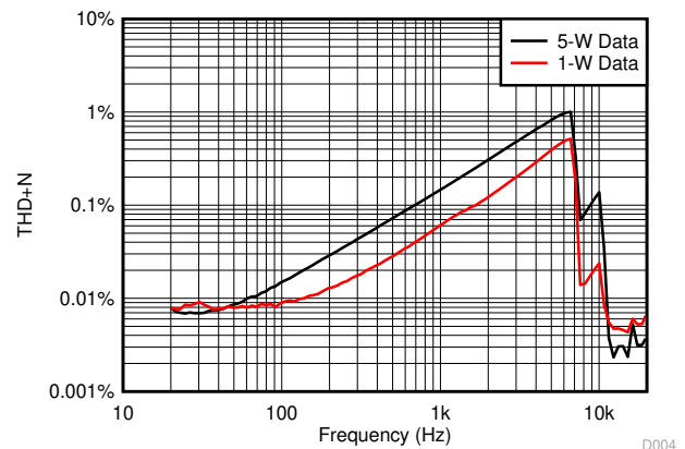
Figure 6-4. THD+N vs Frequency
