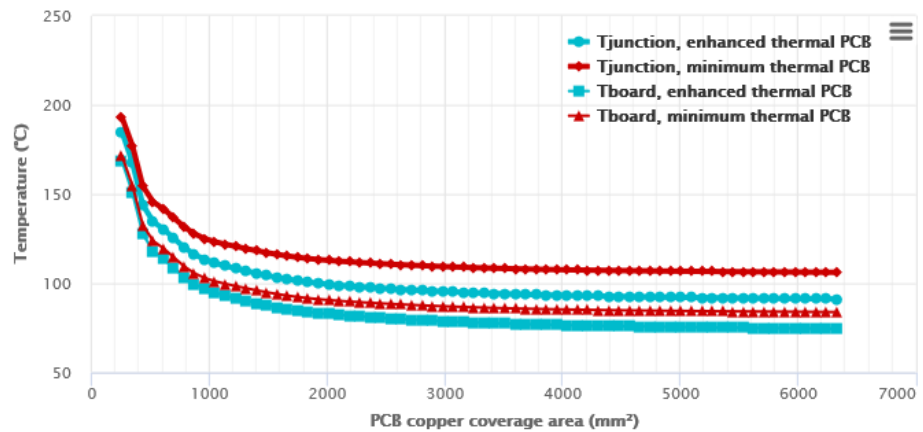
Figure 13. TI PCB Thermal Calculator Example
