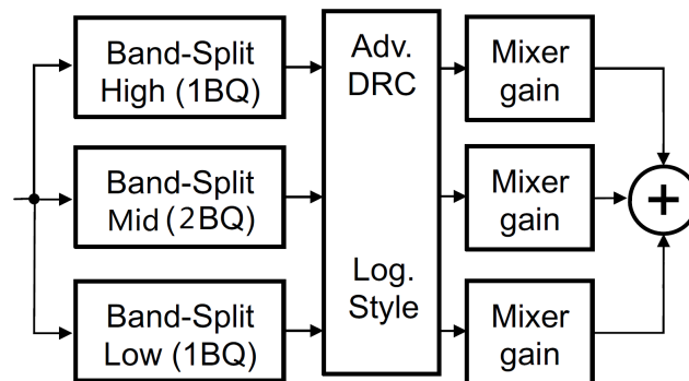
Figure 20. 3-Band DRC
