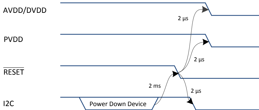
Figure 37. Power-Down Timing
