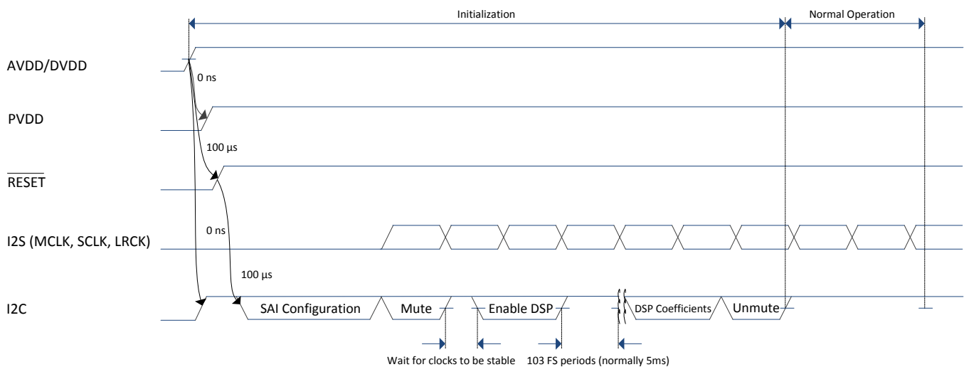
Figure 36. Power-Up Timing
