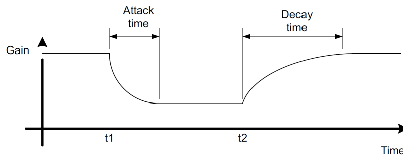
Figure 15. 1-Band DRC Attack and Decay
