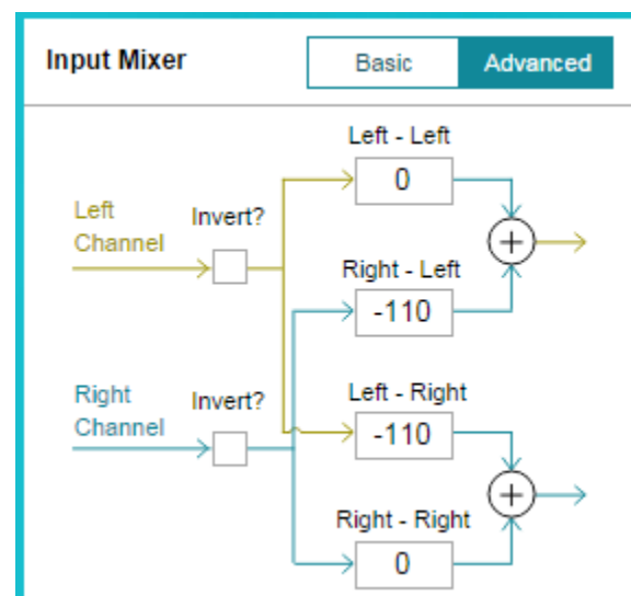
Figure 6. Input Mixer (Advanced Tab)
