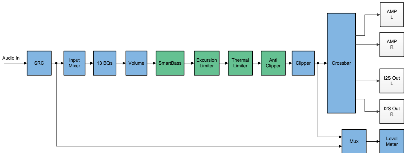
Figure 5. Process Flow 5
