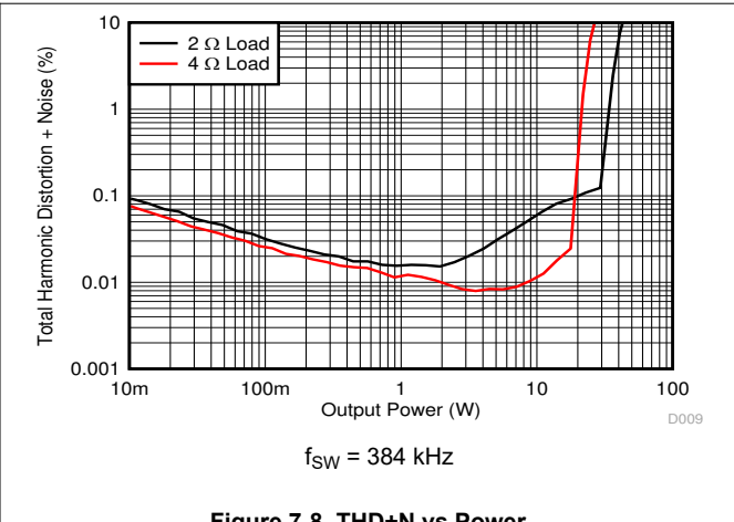
Figure 7-8. THD+N vs Power
