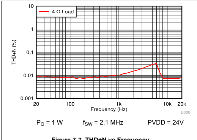
Figure 7-7. THD+N vs Frequency
