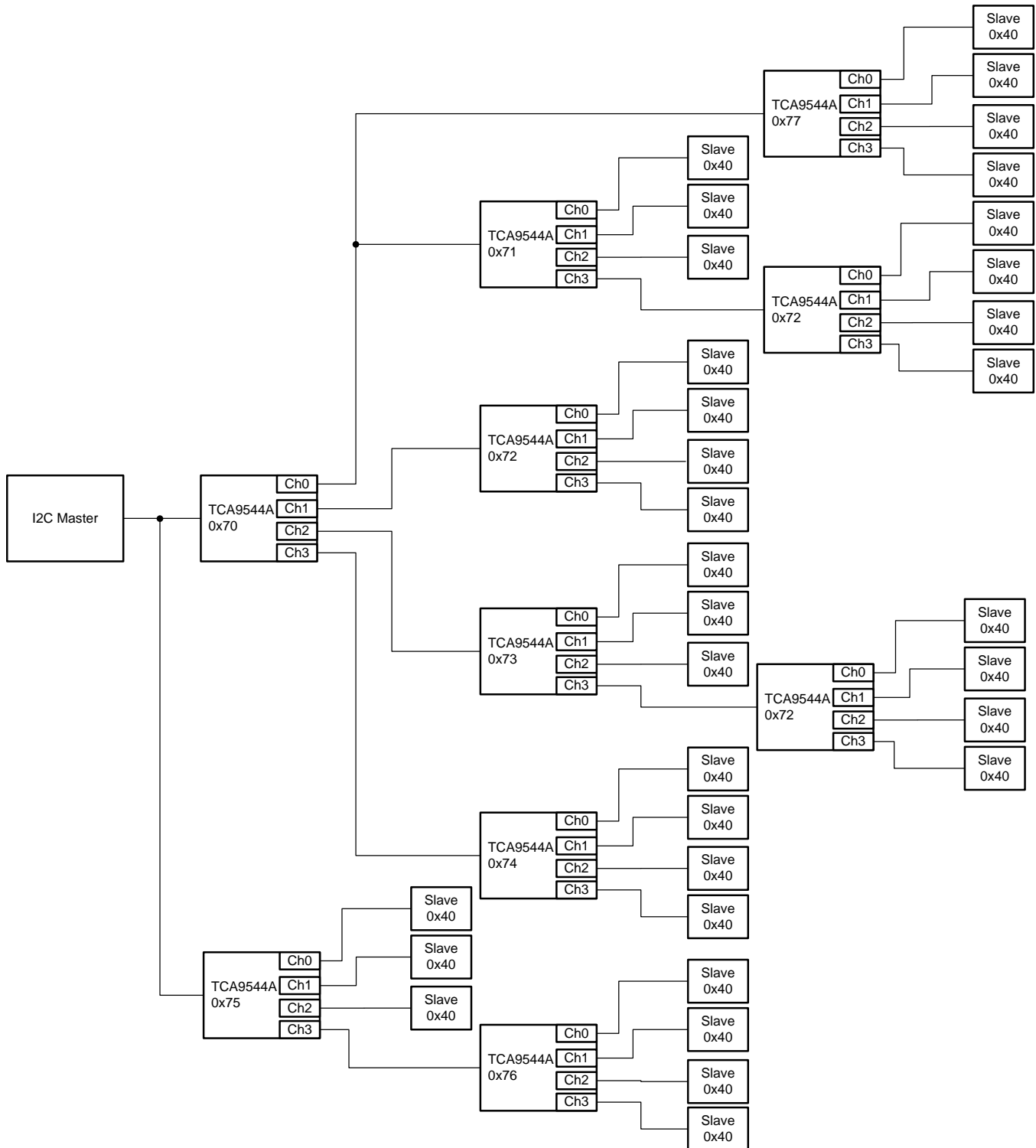
Figure 4. Example of a Complex I2C Tree with Multiple Switches
