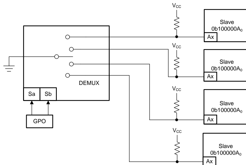
Figure 6. Example of GPO Controlling a MUX
