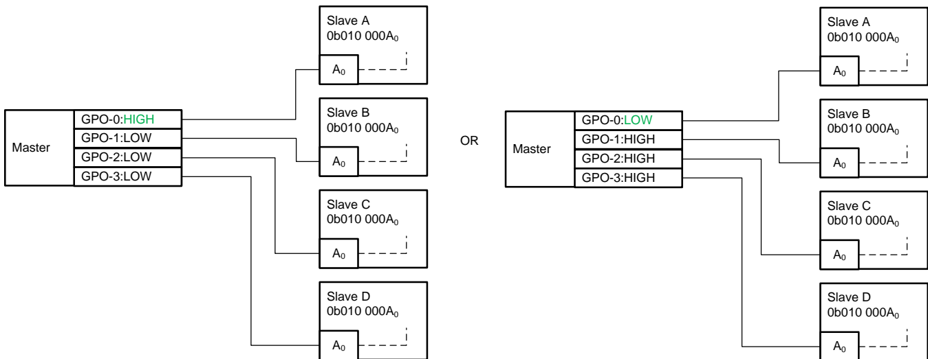
Figure 5. Example of GPOs Controlling Addresses to Communicate with Slave A
