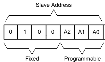
Figure 1. Example of a Three Bit Hardware Addressable I2C Slave (TCA9555)
