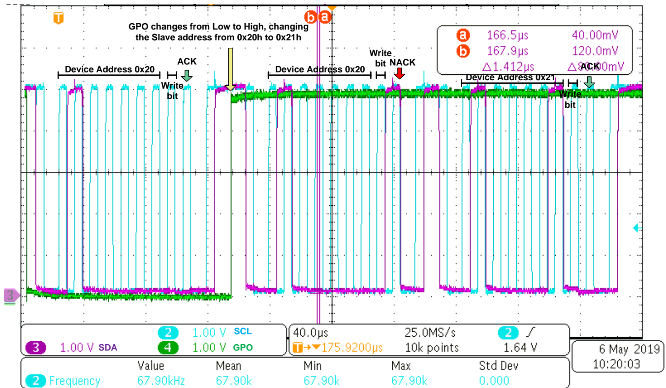
Figure 2. Example Testing to See if TCA6408A Latches Its Address After Power Up
