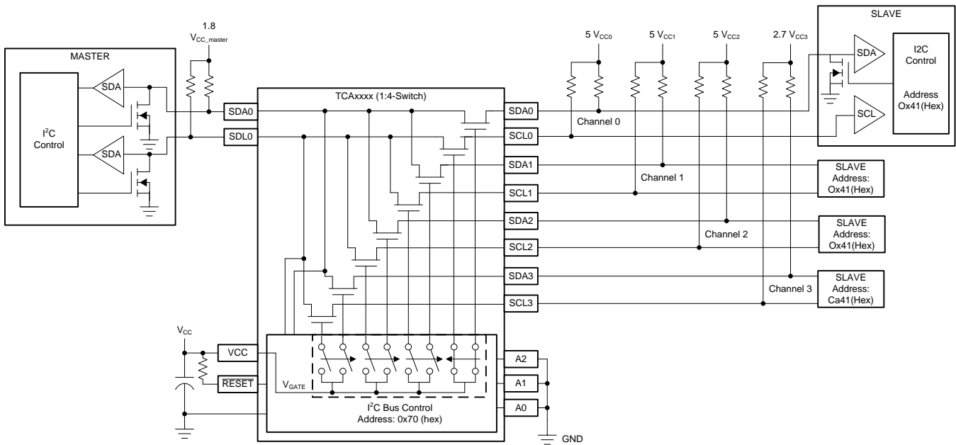
Figure 3. Example of an I2C Switch and How It Switches Internally
