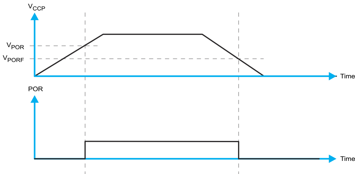
Figure 9-9. V_{POR}
