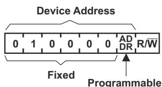
Figure 8-7. TCAL6416 Address
