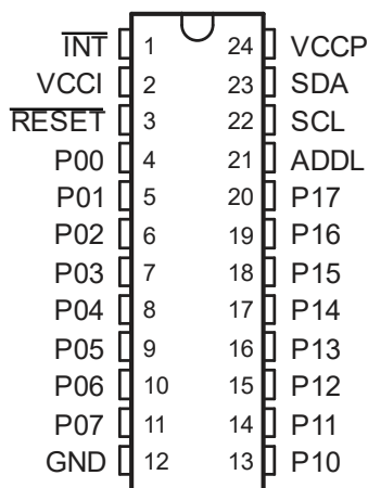
Figure 5-1. PW Package, 24-Pin TSSOP, Top View
