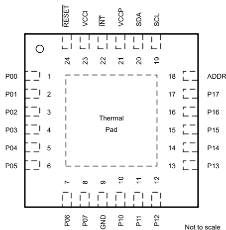
The exposed center pad must be connected as a secondary ground or left electrically open. Figure 5-2. RTW Package, 24-Pin WQFN, Top View
