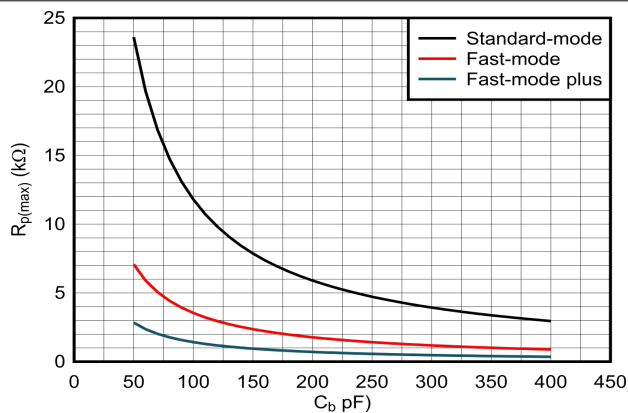
Figure 9-4. Maximum Pullup Resistance ( R_{p(max)} ) vs Bus Capacitance ( C_b )
