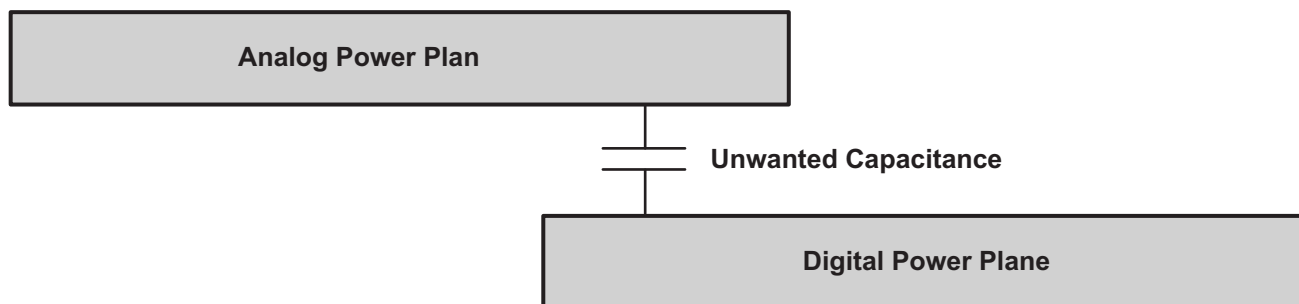
Figure 6. Overlapped Planes
