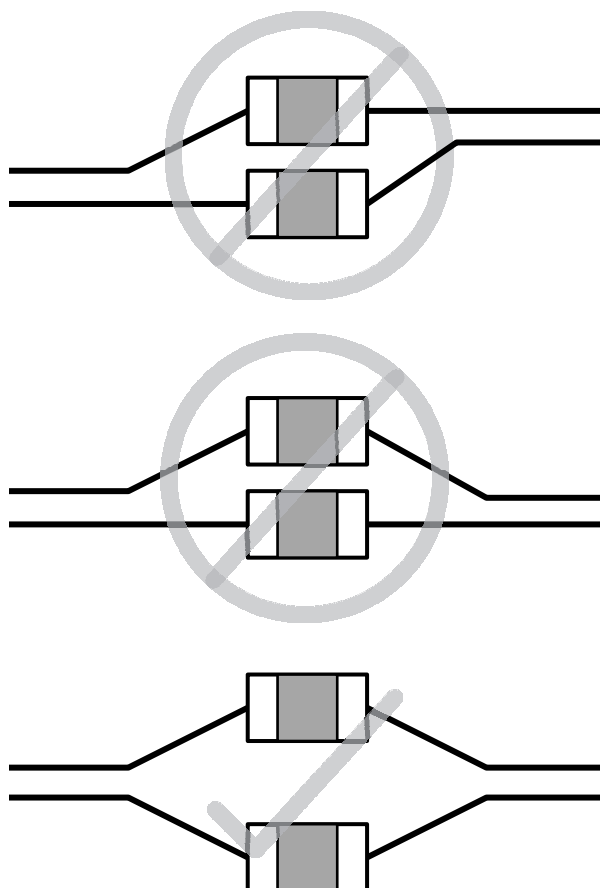
Figure 14. AC-Coupling Placement
