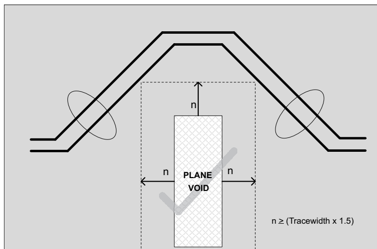
Figure 3. Correct Plane Void Routing
