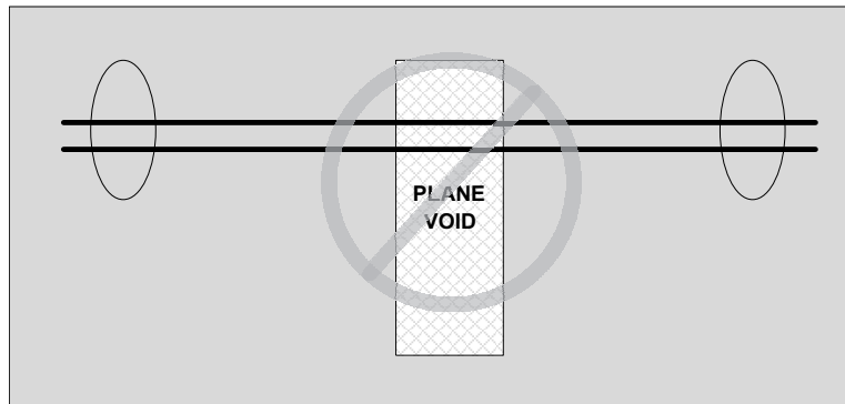
Figure 2. Incorrect Plane Void Routing
