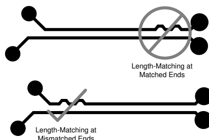
Figure 1. Differential Pair Length Matching
