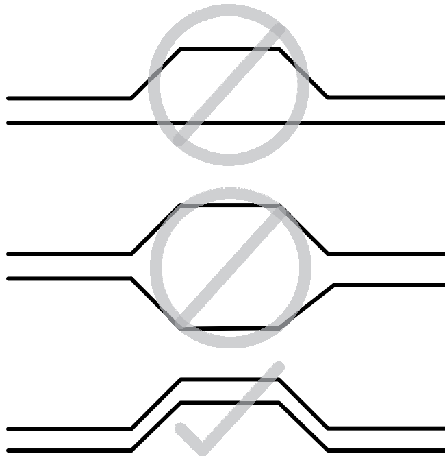
Figure 9. Differential Pair Symmetry
