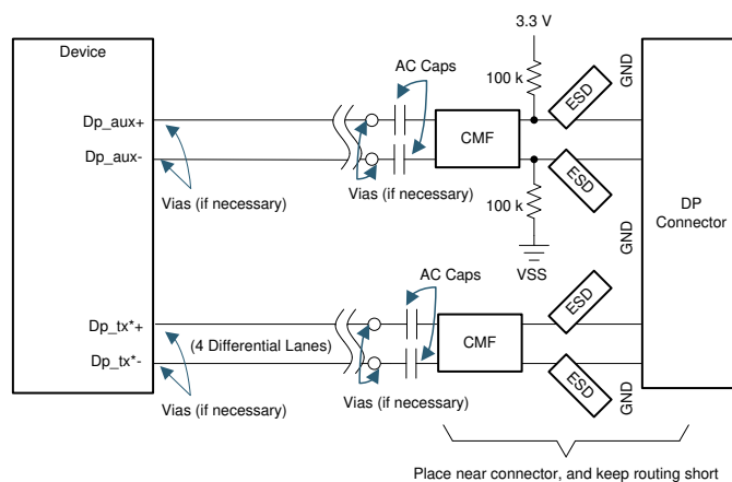
Figure 21. DisplayPort Interface High Level Schematic
