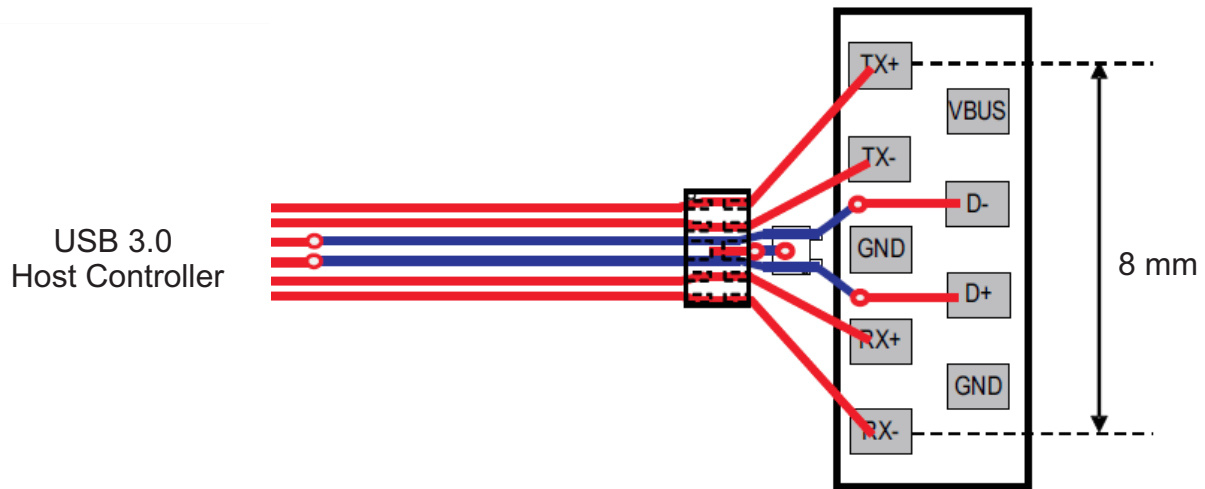
Figure 17. Flow-Through Routing
