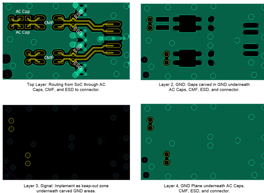
Figure 20. USB 3.1 Example “carve GND” Layout
