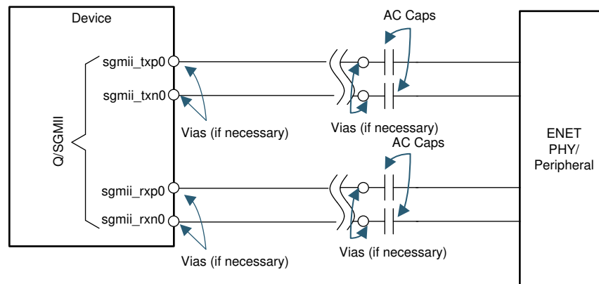
Figure 28. SGMII Interface High Level Schematic
