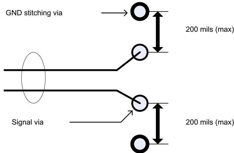
Figure 7. Stitching Vias
