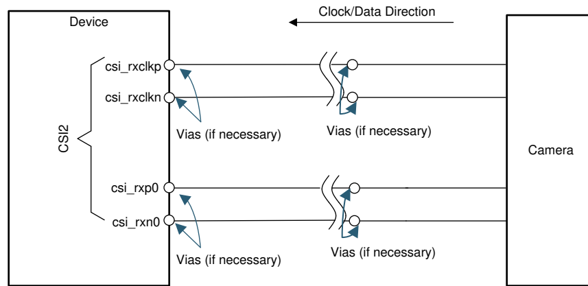
Figure 25. CSI2 Interface High Level Schematic
