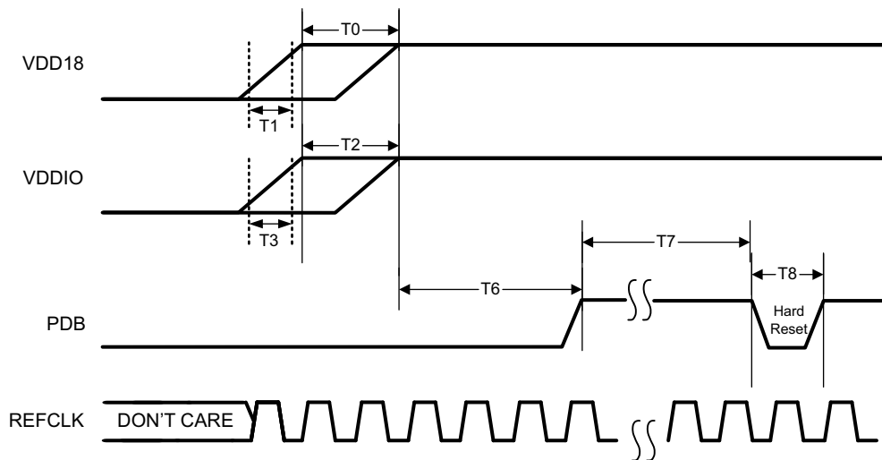
Figure 9-1. Power Supply Sequencing VDD_SEL = LOW, Internal VDD 1.1-V Supply
