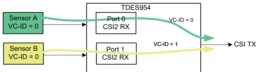
Figure 7-12. VC-ID Mapping Example 1
