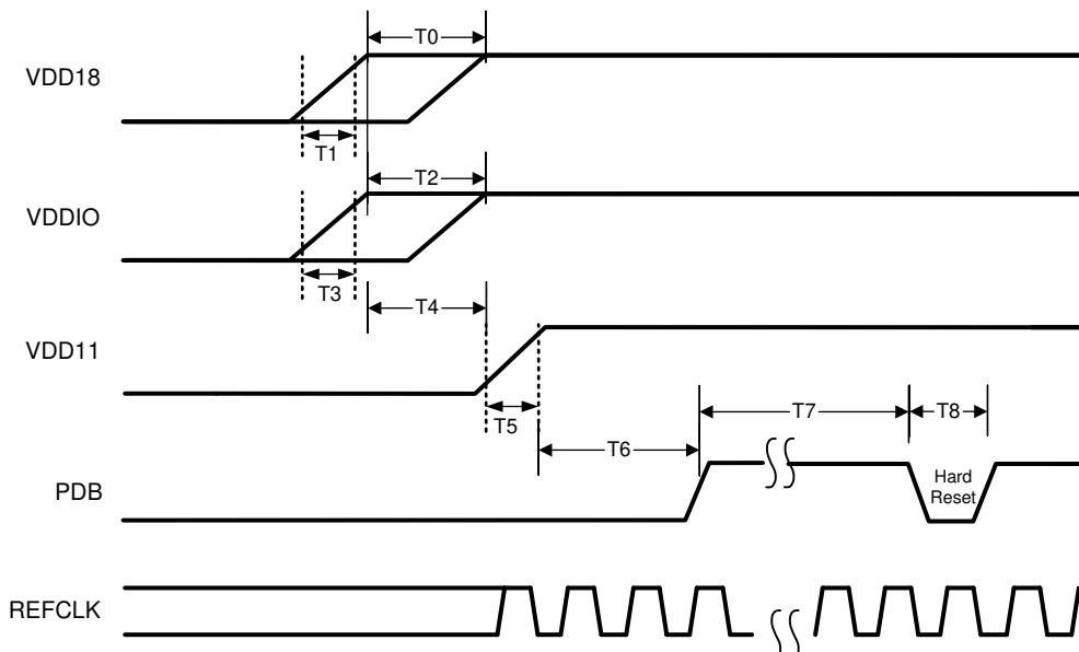
Figure 9-2. Power Supply Sequencing VDD_SEL = HIGH, External VDD 1.1-V Supply
