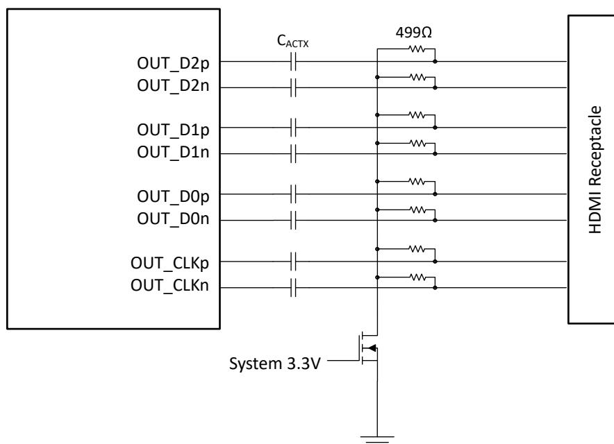
Figure 8-3. AC-Coupled TX in HDMI Source Application (AC_EN = High). External ESD Not Shown.
