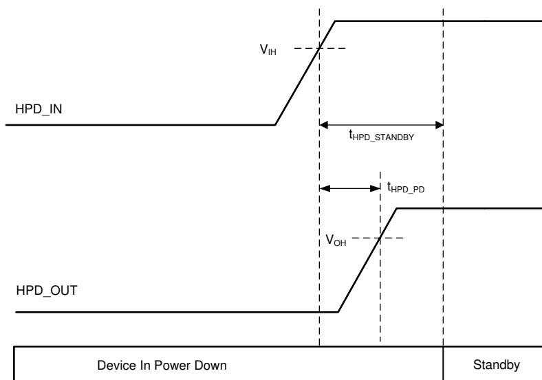
Figure 7-8. HPD Logic Standby and Propagation Timing
