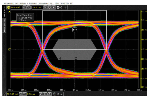
Figure 9-7. 2.97 Gbps Output Eye at TTP4 After Pre and Post Channels
