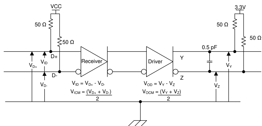
Figure 7-2. TMD5 Main Link Test Circuit
