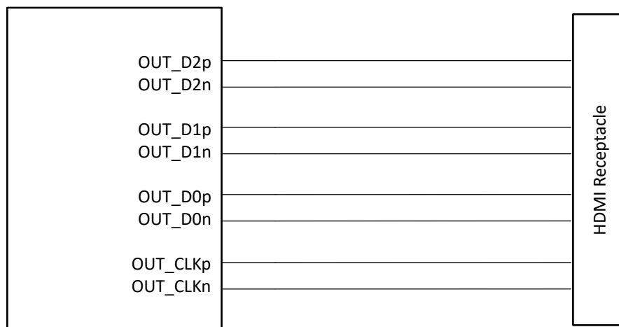
Figure 8-2. DC-Coupled TX in HDMI Source Application (AC_EN = Low). External ESD Not Shown.
