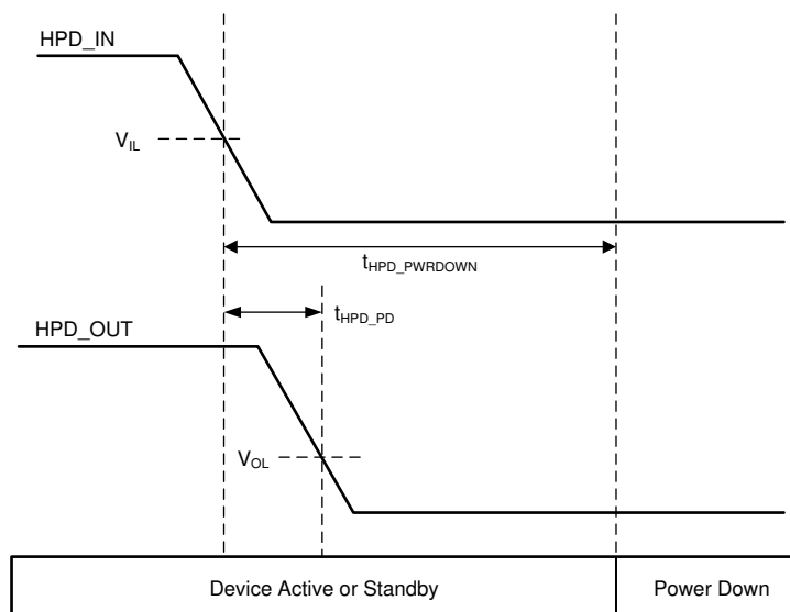
Figure 7-7. HPD Logic Shutdown and Propagation Timing
