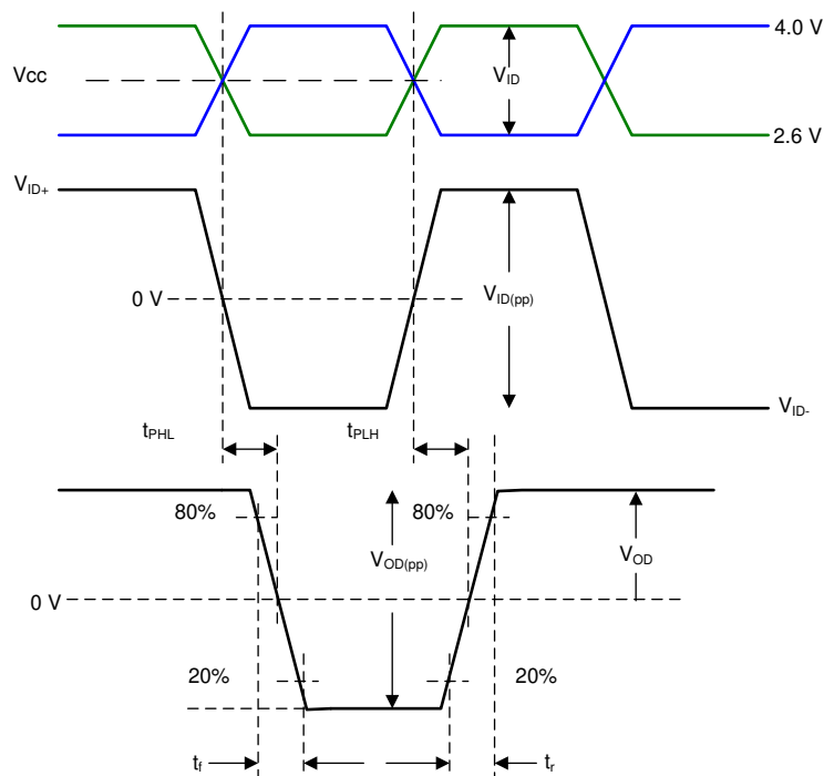
Figure 7-3. Input or Output Timing Measurements
