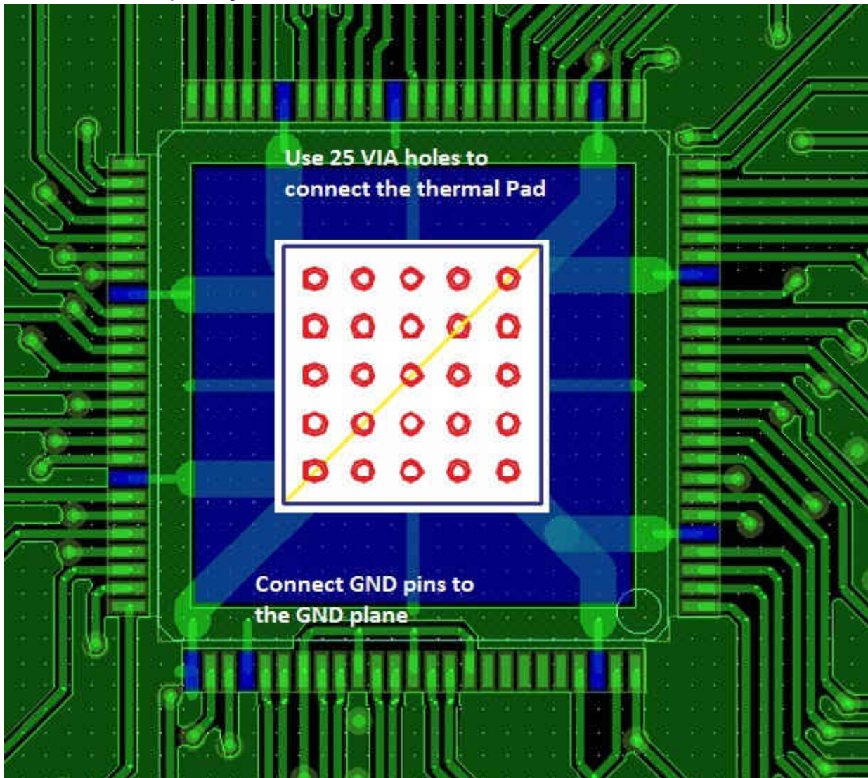
Figure 8-10. GND Route
