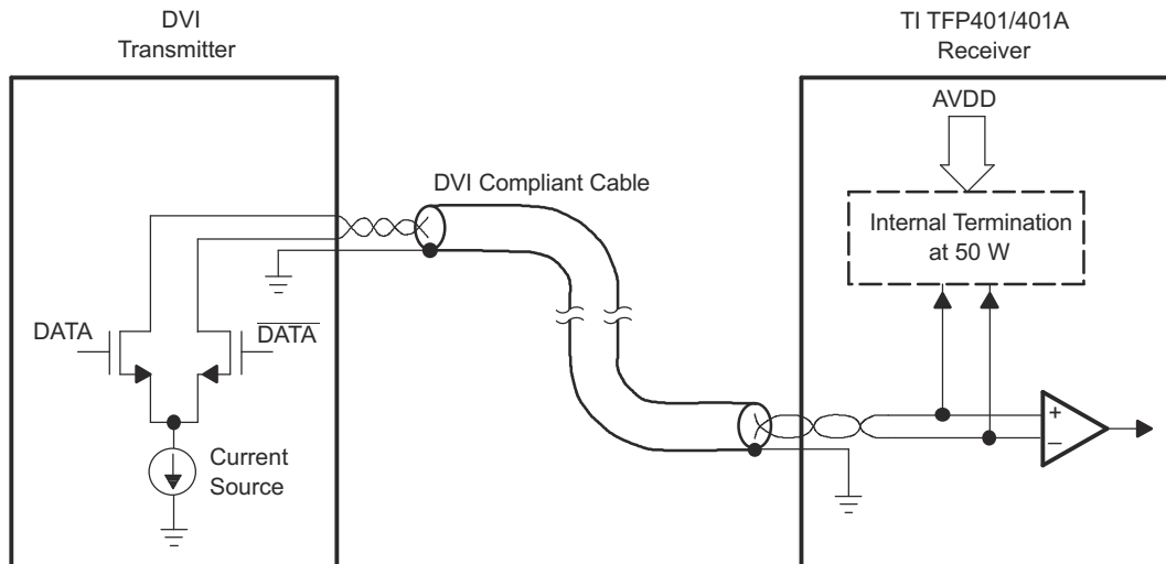
Figure 7-1. TMDS Differential Input and Transmitter Connection
