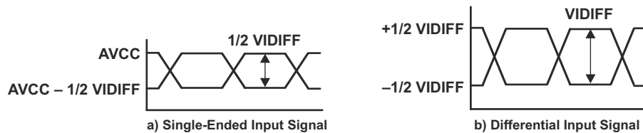
Figure 7-2. TMDS Inputs
