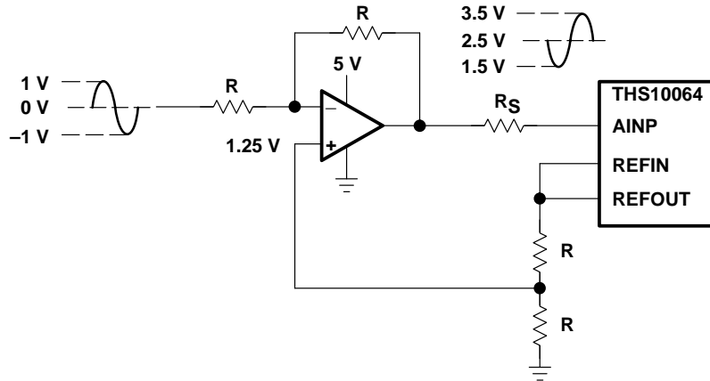
Figure 44. Level-Shift for DC-Coupled Input
