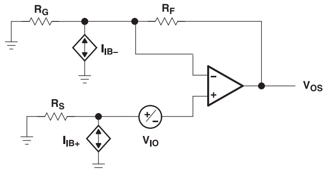
Figure 50. Output Offset Voltage Model
