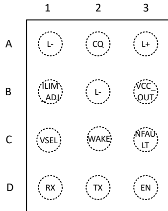
Figure 5-3. TIOL1123 YAH (DSBGA), 12-Pin (Top View)
