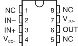
TL971...D PACKAGE (TOP VIEW)
