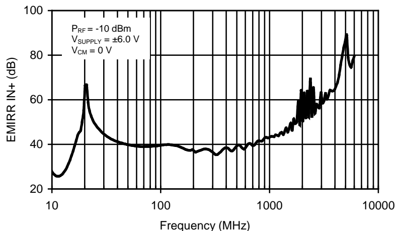
Figure 1. TLC071 EMIRR IN+ vs Frequency
